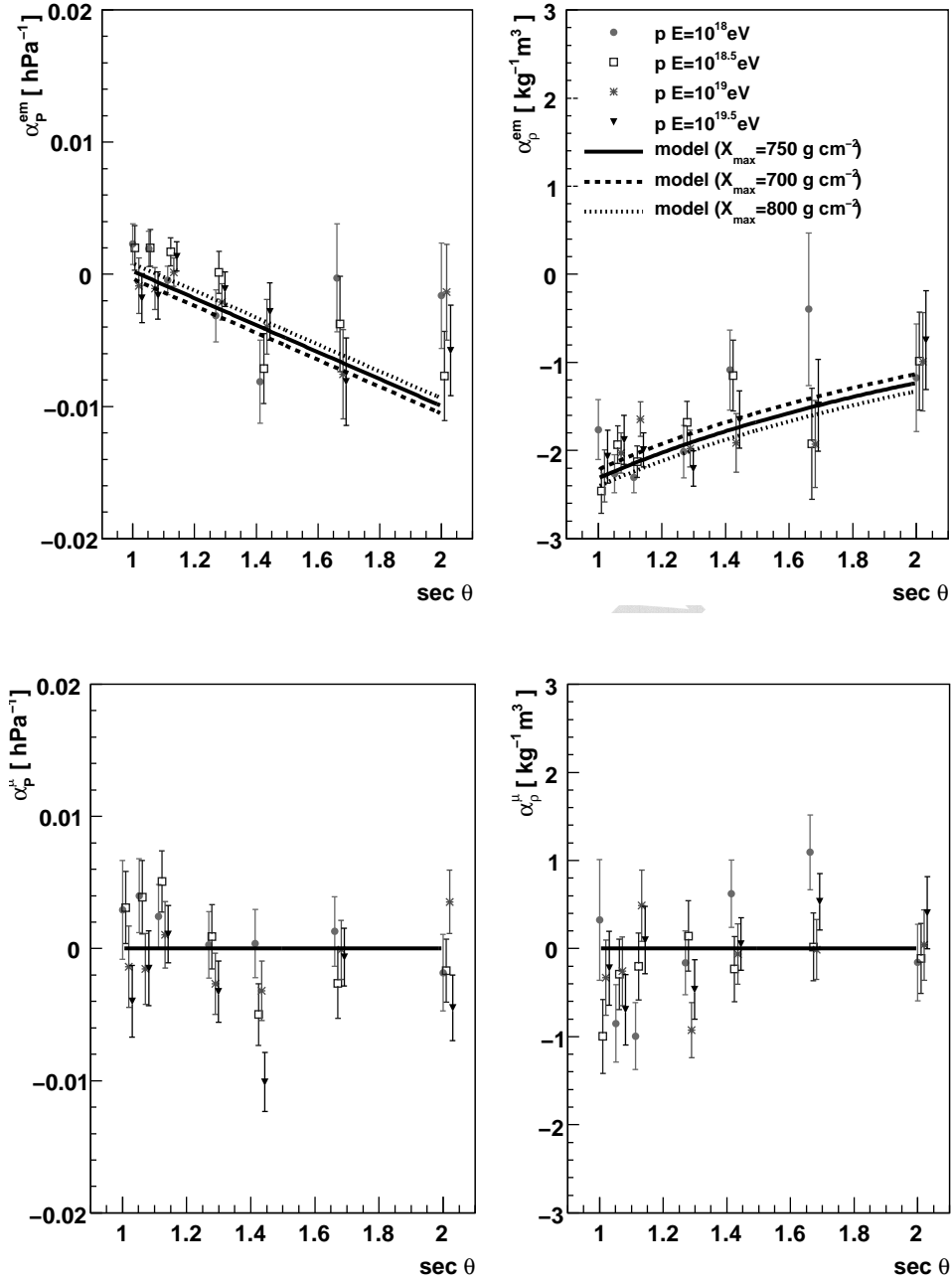
Fig. 7. Top: atmospheric coefficients ( \alpha_P on the left and \alpha_\rho on the right) for the electromagnetic component as a function of \text{sec } \theta . The differently coloured markers correspond to the four simulated energies and the lines represent the model for three different values of X_{\text{max}} . Bottom: \alpha_P (left) and \alpha_\rho (right) for the muonic component as a function of \text{sec } \theta .
