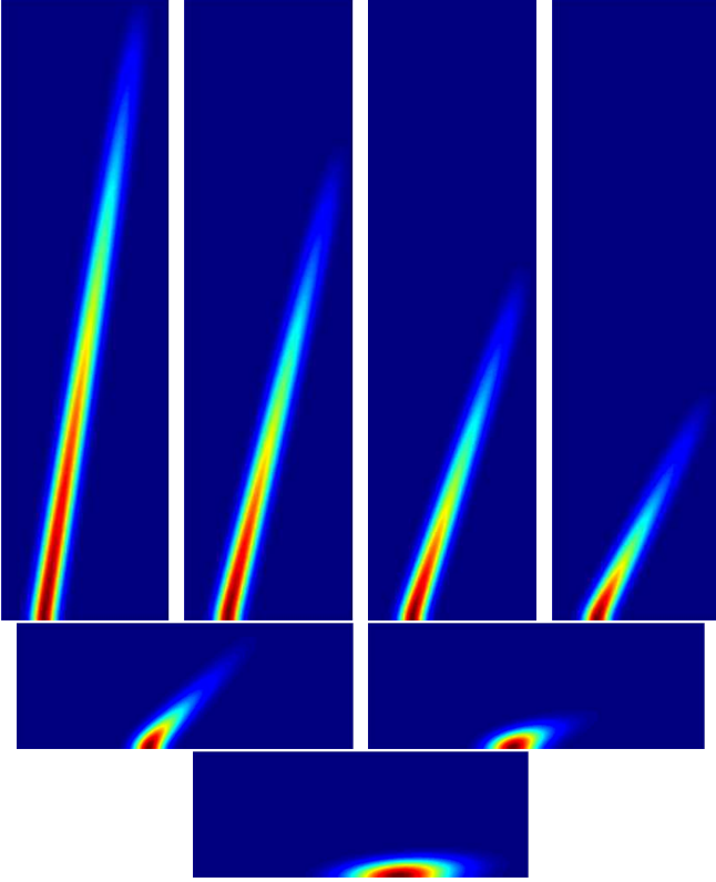
Figure 1: First eigenvector of \mathcal{L}_\theta for \theta = \vartheta\pi/2 with \vartheta = 0.9, 0.85, 0.8, 0.7, 0.5, 0.2, and 0.05, and computed eigenvalues 1.0001, 0.9998, 0.9991, 0.9945, 0.9611, 0.7950, and 0.6481, respectively.
