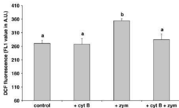
Fig. 3. Comparison of the mean level of ROI/RNI production expressed as DCF fluorescence (FL1 value, in arbitrary unit A.U., n=4+SE ) in C. gigas granulocytes at 120 min incubation at ambient temperature in FSSW (control) or after addition of cytochalasin B (+cyt B: 10 \mu\text{g mL}^{-1} final concentration), zymosan (+zym: 20 particles hemocyte ^{-1} ) or both chemicals (+cyt B +zym) (letters indicate significant differences between conditions, ANOVA, p < 0.05 ).
