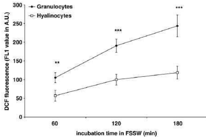
Fig. 1. Comparison of the mean level of ROI/RNI production expressed as DCF fluorescence (FL1 value, in arbitrary unit A.U., n=19+SE ) in C. gigas granulocytes and hyalinocytes at different incubation times (60, 120, 180 min) in FSSW at ambient temperature (Mean comparison: ANOVA; NS: no significant differences, **significant differences at p<0.01 , *** p<0.001 ).
