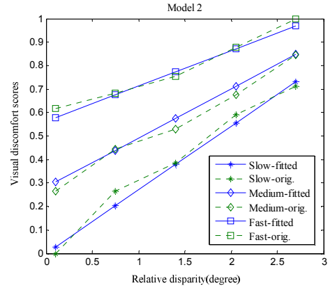
Fig. 10. The predicted visual discomfort of Model 2 in function of disparity and velocity. Solid lines represent fitted scores. Dashed lines represent original normalized Thurstone scores.
