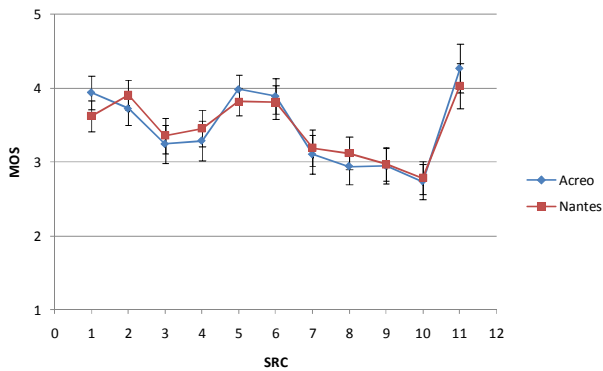
Figure 4: The MOS across SRC of the different laboratories after scaling Lab 2's (Acreo) data to Lab 1 (IRCCyN). The error bars shows 95% confidence intervals
