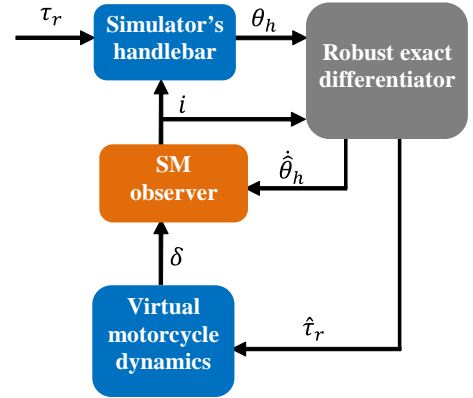
Fig. 6. Diagram for interfacing the virtual motorcycle and the simulator's handlebar
