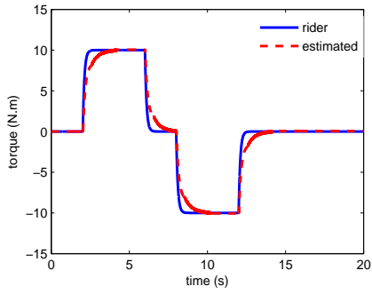
Fig. 7. Estimation of \pm 10 (N.m) unknown input torque
