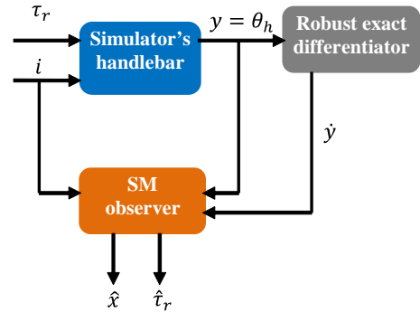
Fig. 3. Unknown input sliding observer diagram
