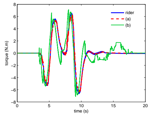
Fig. 13. Comparison between the VGSTA (a) and an H_\infty control (b) performance for a double lane change at 40(km/h)
