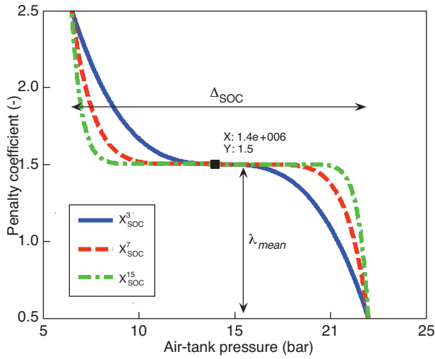
Figure 9 Non-linear function of variable penalty coefficient.
