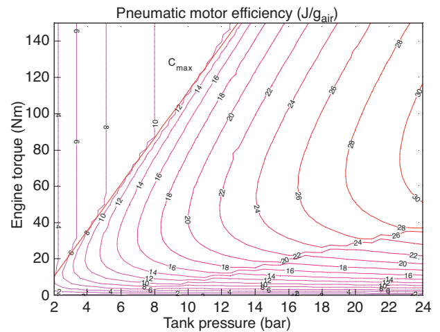
Figure 7 Pneumatic motor performance ( J/g_{air} ) versus engine torque (Nm) and tank pressure (bar).
