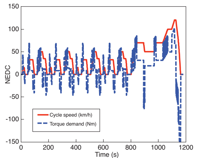
Figure 2 NEDC driving cycle.
