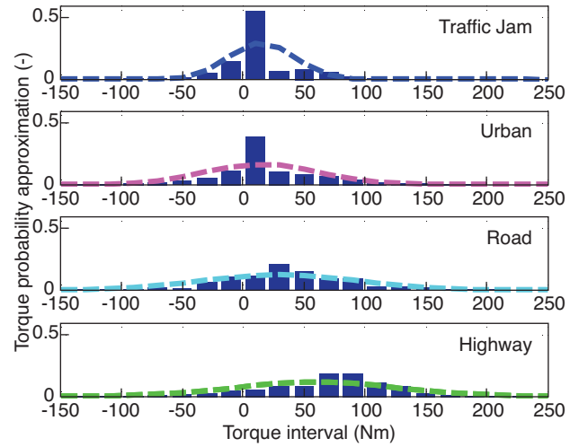
Figure 10 Patterns as probability density of Artemis driving cycles.
