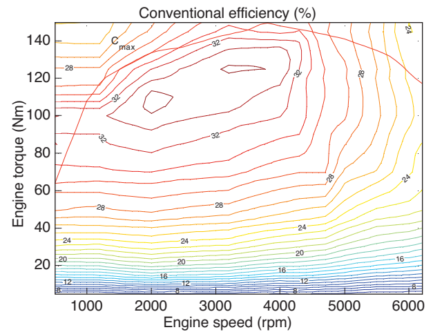
Figure 6 Conventional engine efficiency (%) versus engine torque (Nm) and speed (rpm).
