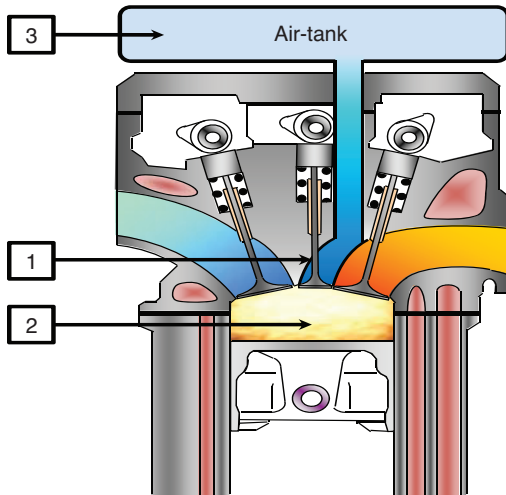
Figure 1 Pneumatic-hybrid scheme.
