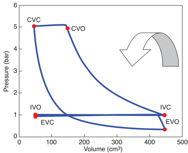
Figure 5 Pump mode indicator diagram.
