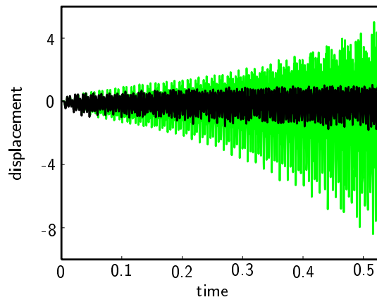
Figure 17: RADIAL DISPLACEMENT OF THE FIRST CONTACT NODE OF THE BLADE AT f_{\Omega} = 0.190 FOR \theta = 0 RAD (—) AND \theta = 0.15 RAD (—).
