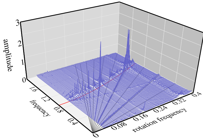
Figure 16: BLADE RESPONSE SPECTRUM FOR \theta = 0.15 RAD.
