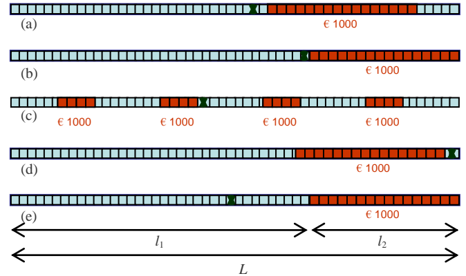
Figure 2: One-dimensional lottery.
