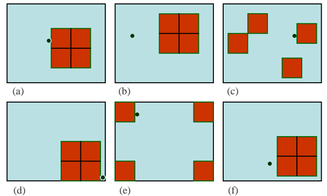
Figure 4: Two-dimensional lottery.
