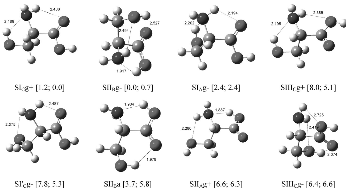
Fig. 2 Optimized geometries (B3LYP/6-31G(2df,p)) of the eight most stable conformers of neutral L-serine (in brackets, relative H_{298}^0 and G_{298}^0 in kJ mol -1 calculated at the G4 level).
