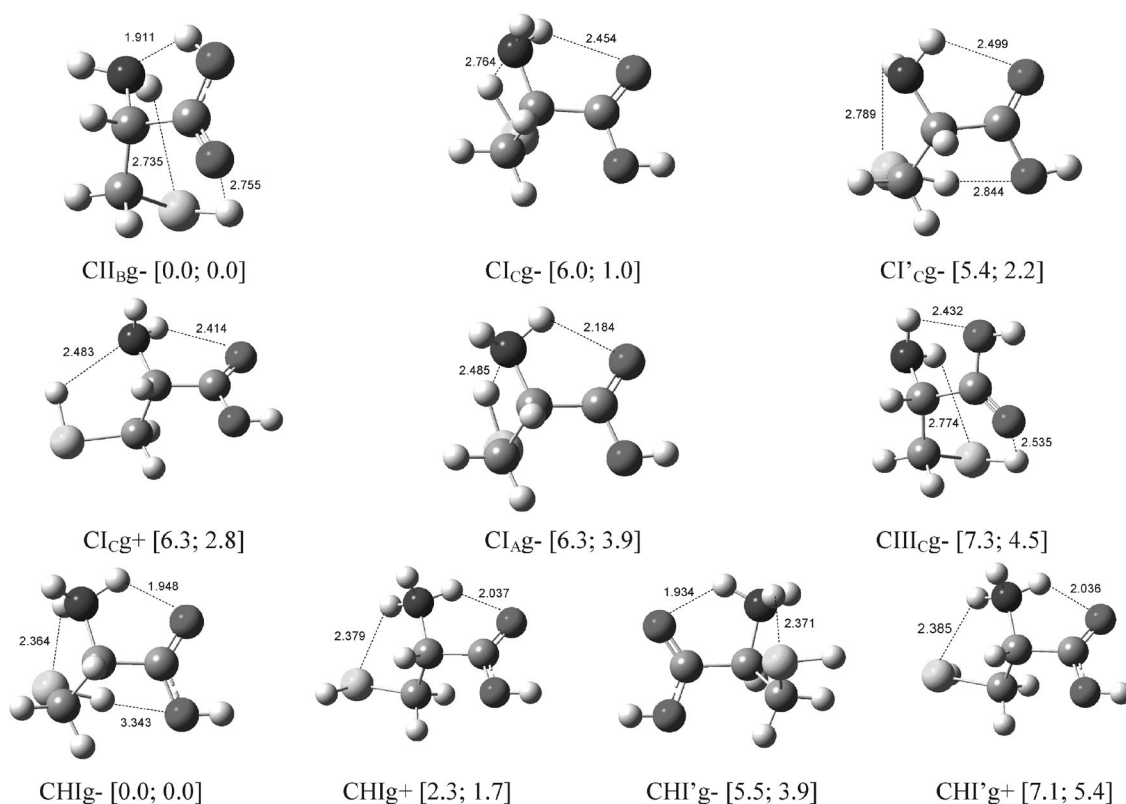
Fig. 8 Optimized geometries (B3LYP/6-31G(2df,p)) of the six stable conformer of neutral L-cysteine and the four most stable conformers protonated L-cysteine (in brackets, relative H_{298}^0 and G_{298}^0 in \text{kJ mol}^{-1} calculated at the G4 level).
