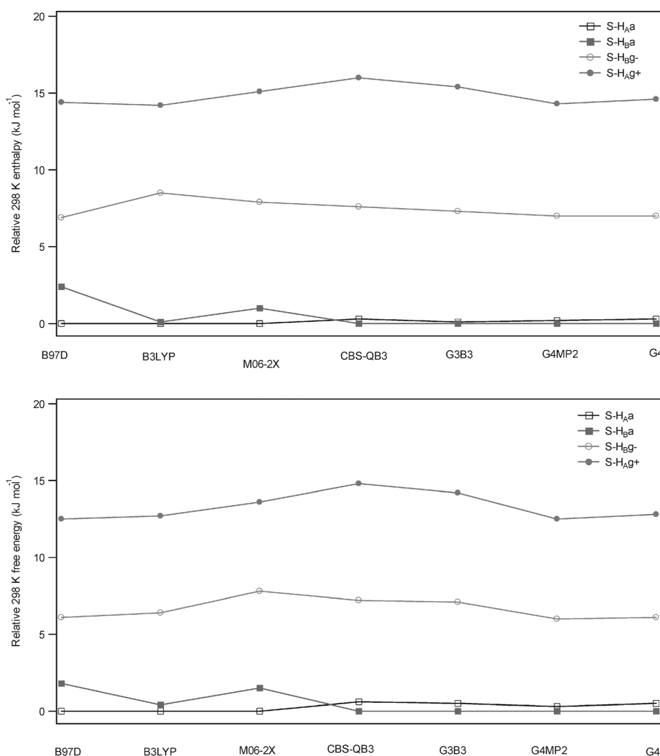
Fig. 5 Relative H_{298}^{\circ} and G_{298}^{\circ} (kJ mol -1 ) of the four most stable conformers of deprotonated L-serine.
