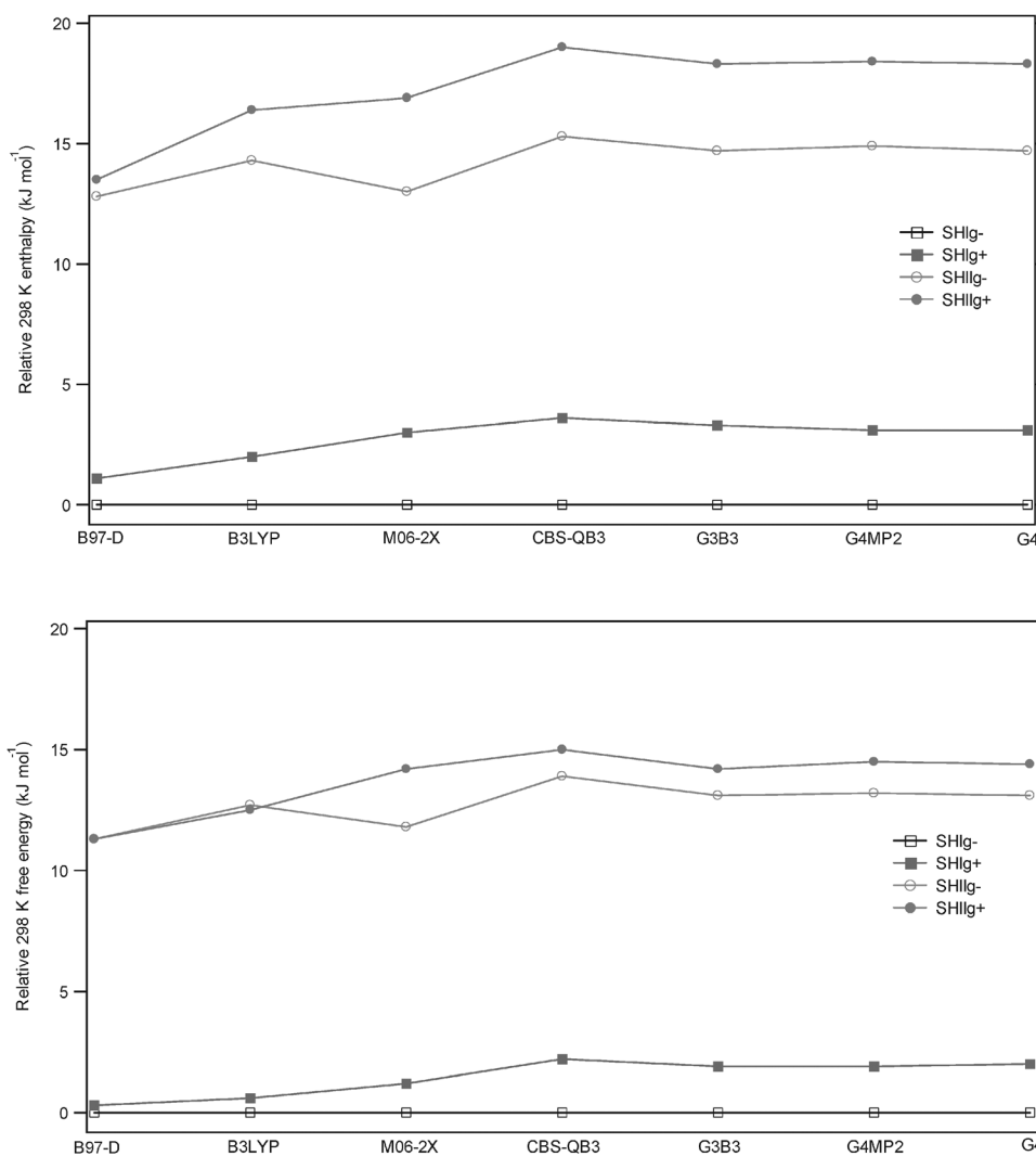
Fig. 3 Relative H_{298}^0 and G_{298}^0 (kJ mol -1 ) of the four most stable conformers of protonated L-serine.
