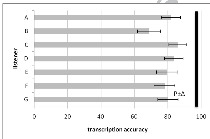
Figure 10: Evaluation of the synthesized speech intelligibility when the phonetic prediction is correct (transcription accuracy and confidence interval). The black vertical bar indicates the average transcription accuracy of the original sentences (97%).
