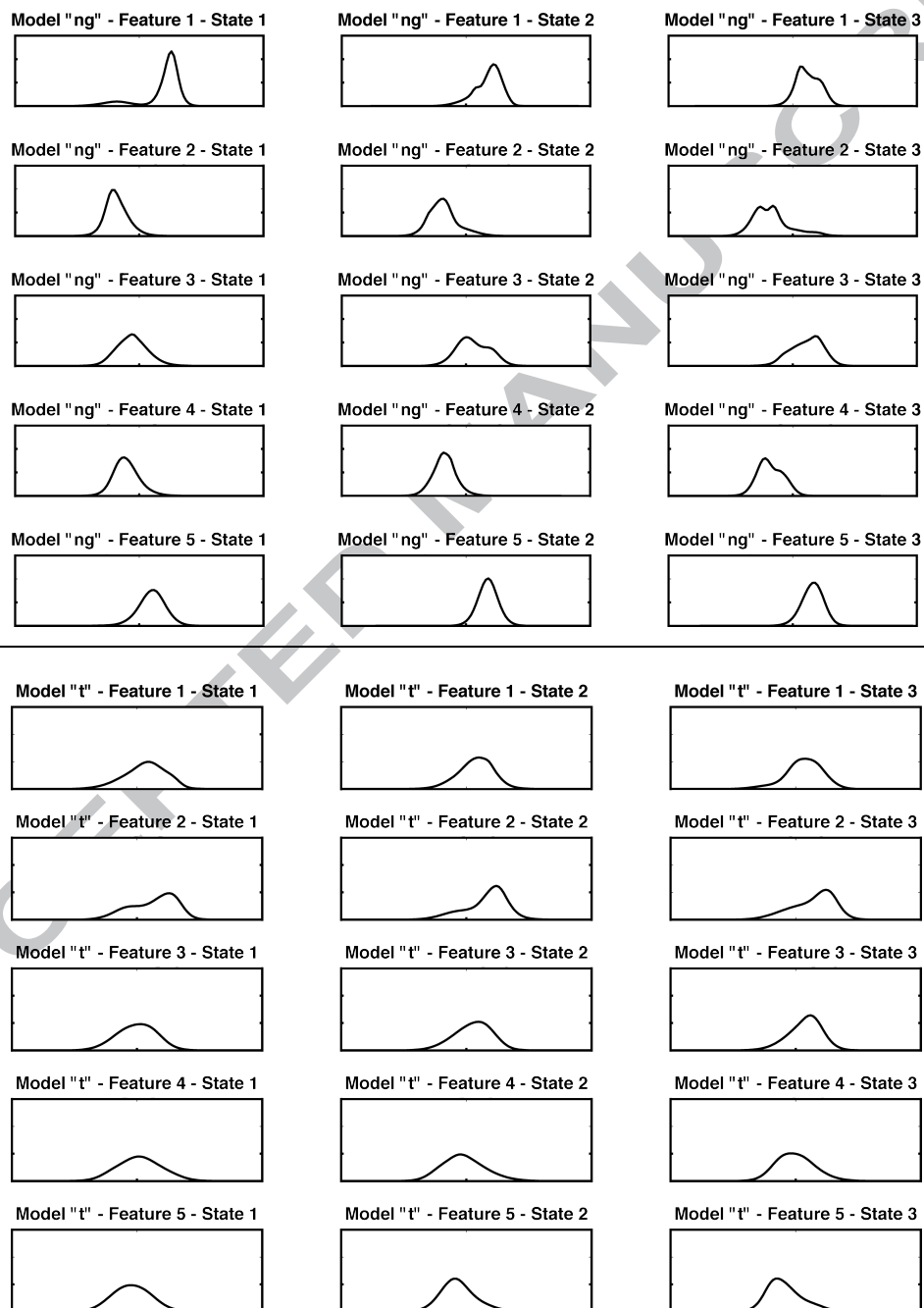
Figure 6: Estimated probability density function for the 5 first EigenTongues coefficients (referred as « Feature ») of the 3 emitting HMM states, for the phone [ng] (top) and phone [t] (bottom).
