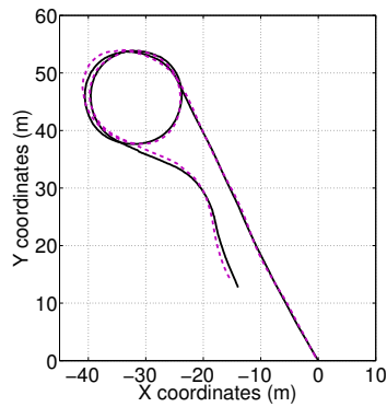
Fig. 8. Tracked path
