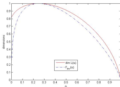
FIGURE 2. When f_1(x) = f_2(x) = x_1 .
