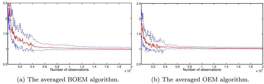
Figure 4: Estimation of x_1 using the averaged OEM and the averaged BOEM algorithms. Each plot displays the empirical median (bold line) and the first and last quartiles (dotted lines) over 100 independent Monte Carlo runs with \tau_n = n^{1.1} and \gamma_n = n^{-0.53} . The first ten observations are omitted for a better visibility.
