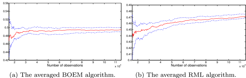
Figure 5: Empirical median (bold line) and first and last quartiles (dotted line) for the estimation of m(1,1) using the averaged RML algorithm (right) and the averaged BOEM algorithm (left). The true values is m(1,1) = 0.5 and the averaging procedure is starter after 10000 observations. The first 10000 observations are not displayed for a better clarity.
