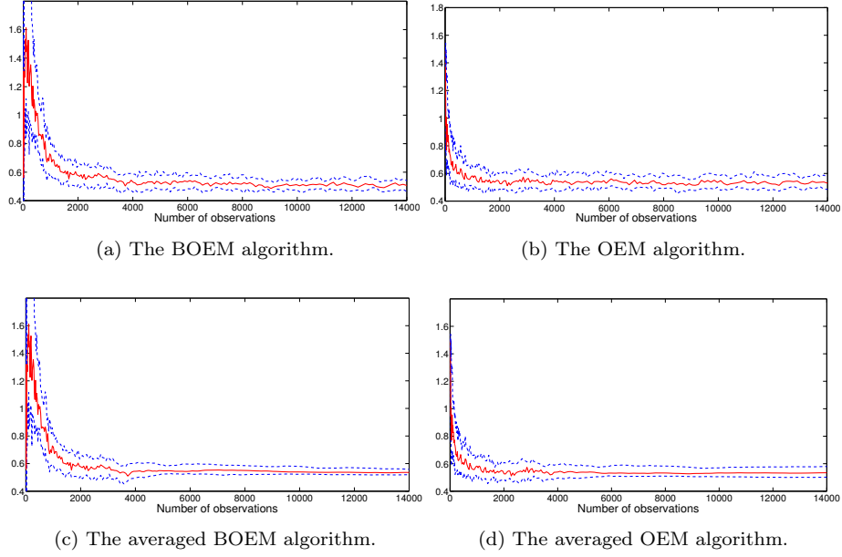
Figure 3: Estimation of v using the online EM and the BOEM algorithms (top) and their averaged versions (bottom). Each plot displays the empirical median (bold line) and the first and last quartiles (dotted lines) over 100 independent Monte Carlo runs with \tau_n = n^{1.1} and \gamma_n = n^{-0.53} .
