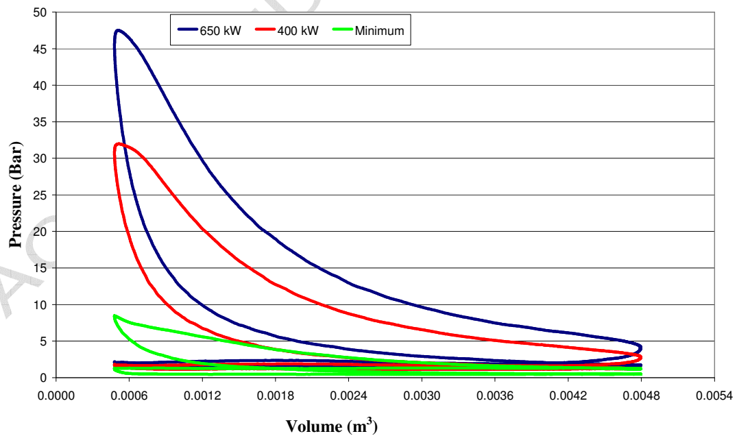
Figure 3 – CAT G3516 LETA: mean indicated cycle at different engine loads
