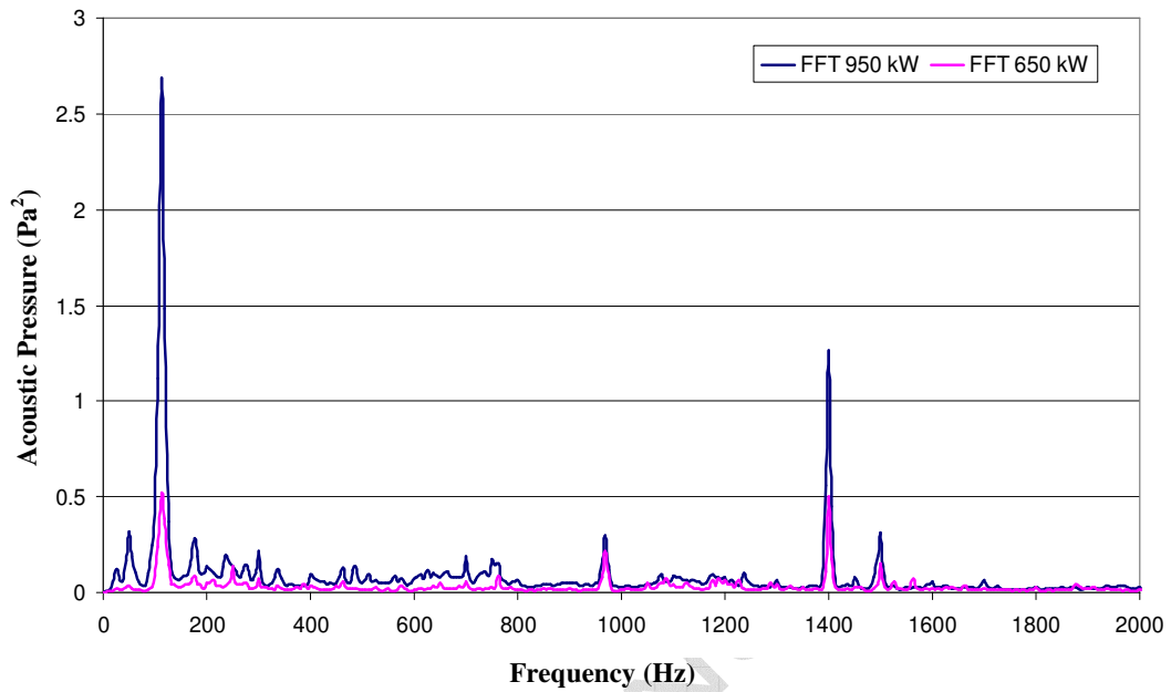
Figure 8 – Acoustic pressure trend in the frequency domain for the load configurations of 950 and 650 kW (CAT G3516B)
