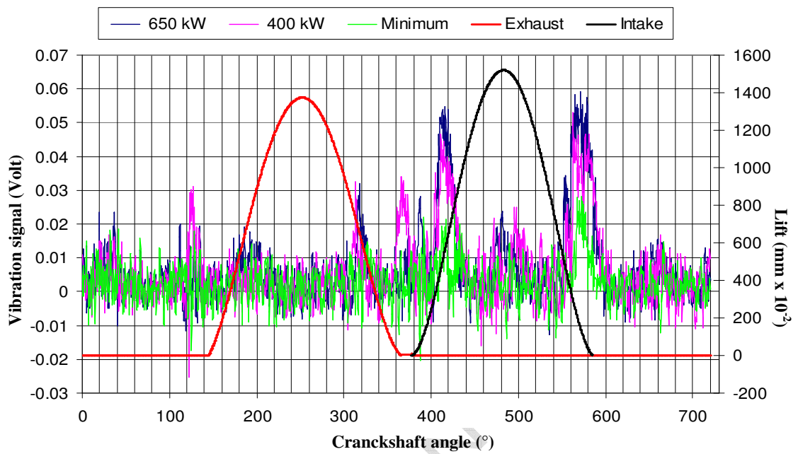
Figure 10 – Inverse value of the vibration signal recorded on the cylinder (CAT G3516 Leta engine) and valves lift law
