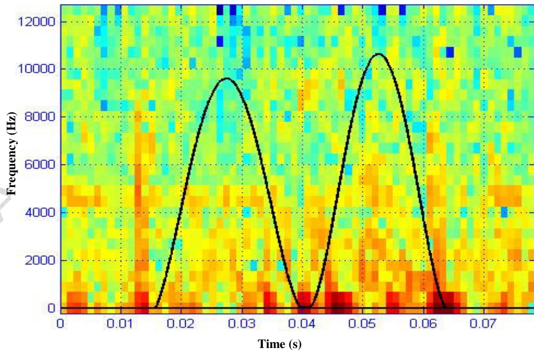
Figure 11 - CAT G3516 LETA spectrograph (400 kW) and valves lift law
