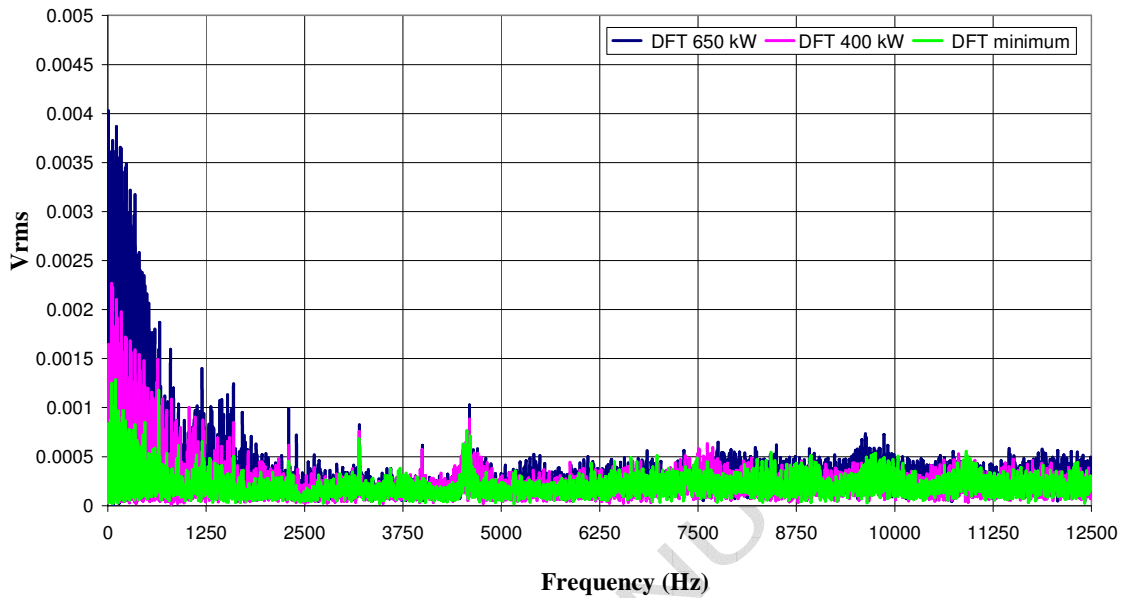
Figure 6 – DFT of the vibration signal
