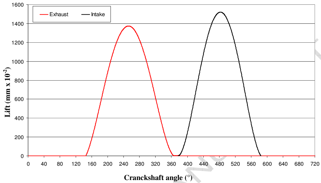
Figure 2 - CAT G3516 LETA: lift law of the intake and exhaust valves
