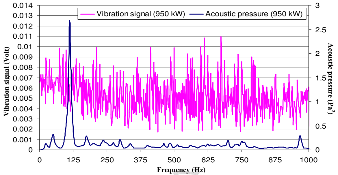
Figure 12 - Comparison between the vibration signal at 950 kW load and the corresponding acoustic pressure
