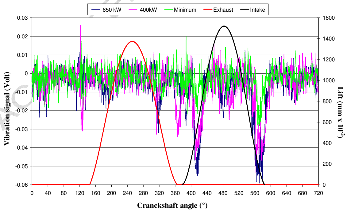
Figure 9 - Vibration trends recorded on the cylinder (CAT G3516 Leta engine) and valves lift law
