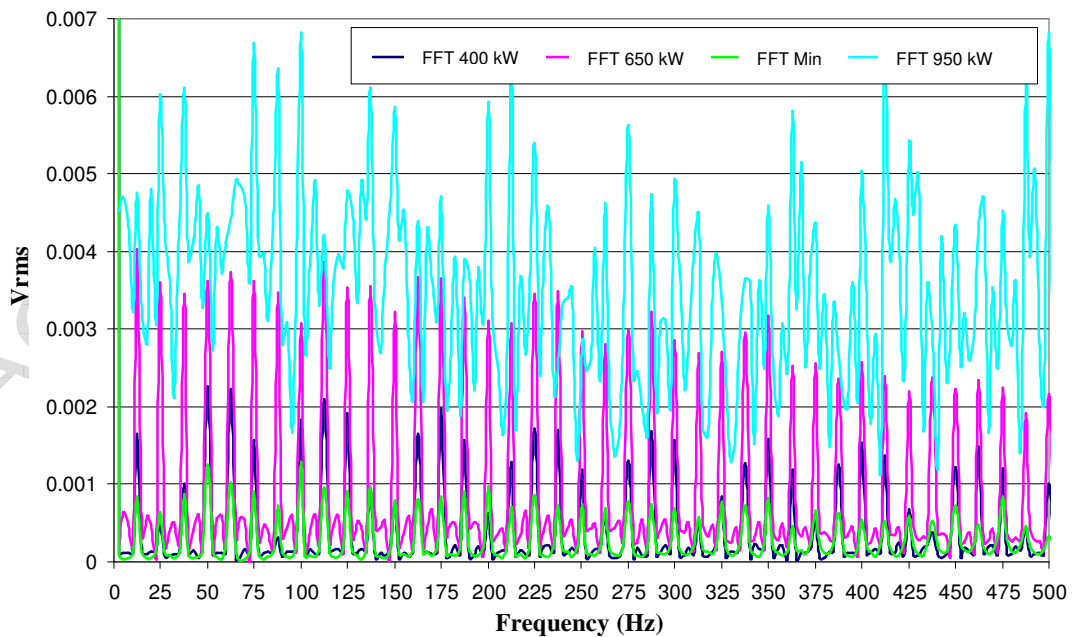
Figure 7 – Comparison between the cylinder head state of vibration (in the frequency domain) of CAT G3516 LETA and CAT G3516B
