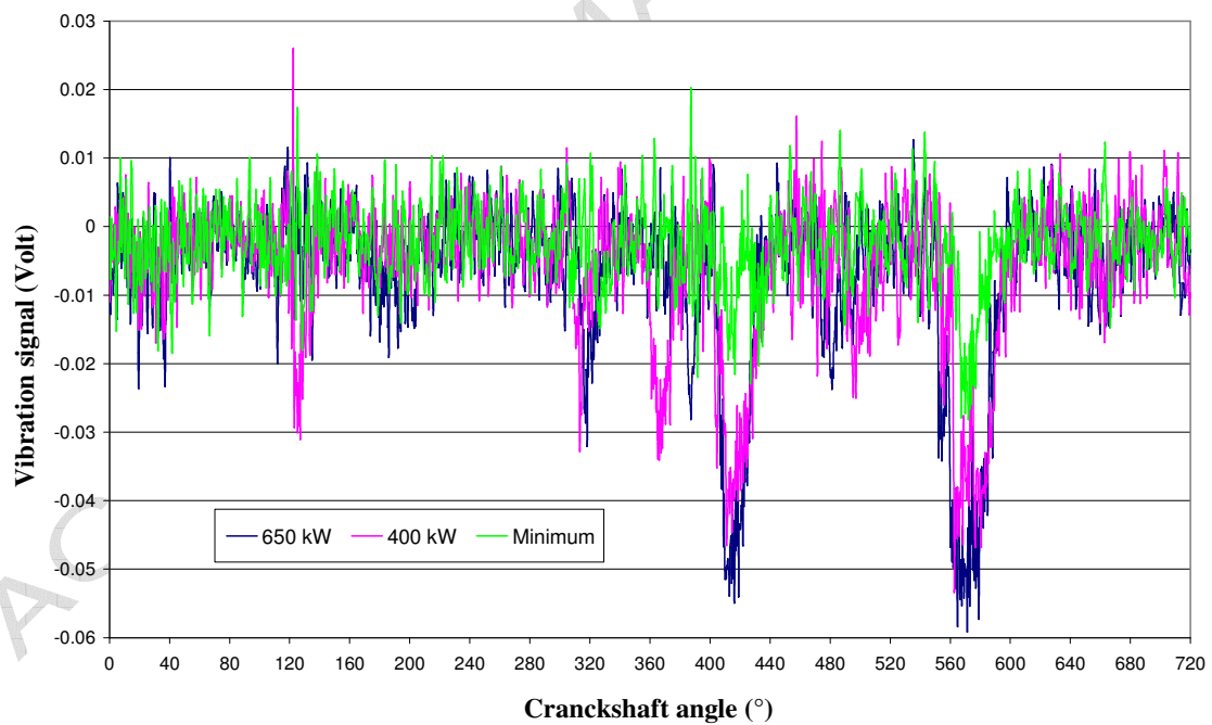
Figure 4 – Vibration and acoustic signal acquisition on the cylinder n. 9 of the CAT G3516B engine
