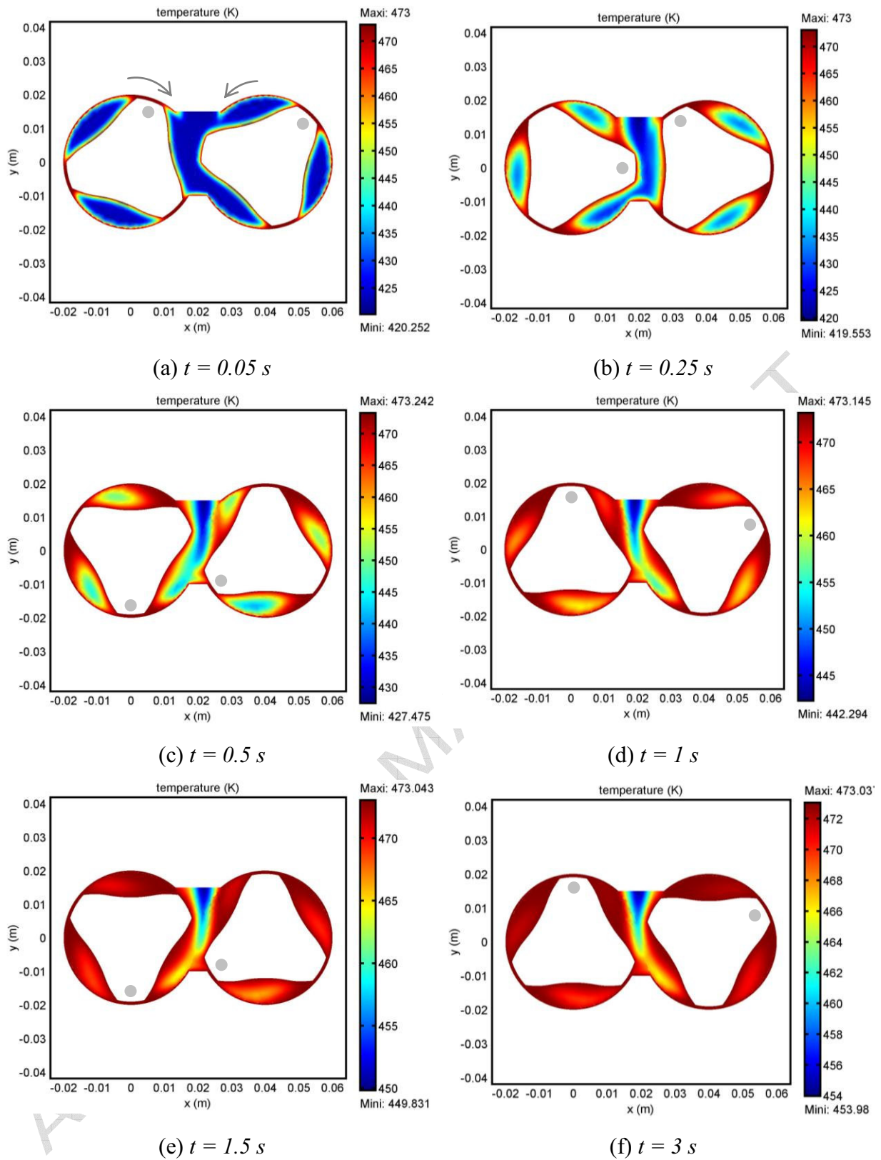
Fig. 14: Temperature field (in K) at several time step for the PP/MWCNT composite with 8 wt% in MWCNT.
