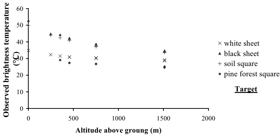
Figure 3. Observed brightness temperatures of the different targets at different altitudes above ground level.
