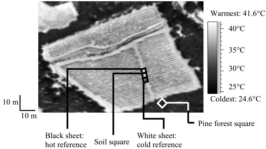
Figure 1. Brightness temperature image of the experimental vineyard and reference targets collected at 750 m altitude above ground.
