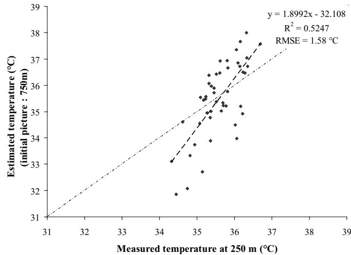
Figure 4. Scatter plot and regression line of estimated (image altitude 750 m) against observed (image altitude 250 m) canopy temperature
