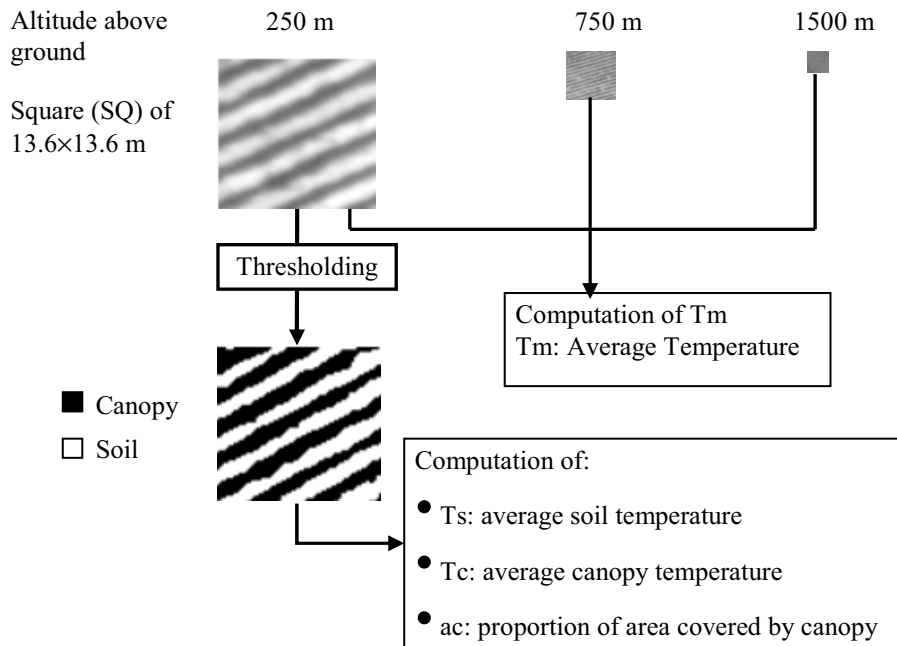
Figure 2. Method used to study the effect of mixed pixels
