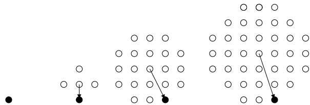
Fig. 1. Translation vectors
