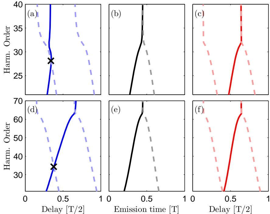
Figure 3. Quantum mechanical in situ phases, \phi_0^{(n)} , between the fundamental and weak second harmonic field that maximize the even harmonic emission in argon ( I_p^{(Ar)} = 15.75 eV) for intensities of (a) 1.5 \times 10^{14} W/cm 2 and (d) I = 4 \times 10^{14} W/cm 2 . The in situ phases are presented as delays, \tau_0^{(n)} = -\phi_0^{(n)}/2\omega in units of T/2 . The corresponding high-order harmonic emission times are shown in (b) and (e), in units of T . Classical in situ phases ( I_p^{(0)} = 0 ) for intensities of (c) 1.5 \times 10^{14} W/cm 2 and (f) I = 4 \times 10^{14} W/cm 2 . The short (long) branch is a full (dashed) curve. T = 2\pi/\omega is the period of the fundamental laser field.
