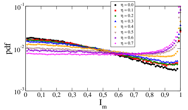
FIG. 10: Probability distribution function of the friction mobilization index I_m .
