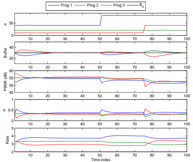
FIG. 3: Study of the equilibrium of the proposed system using a PI controller
