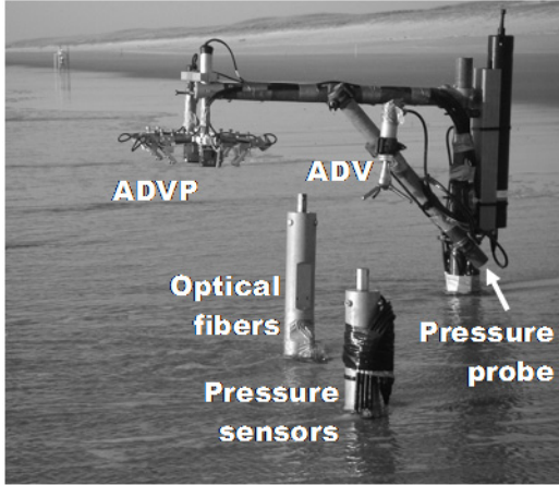
Figure 1. Experimental devices shown at low tide
