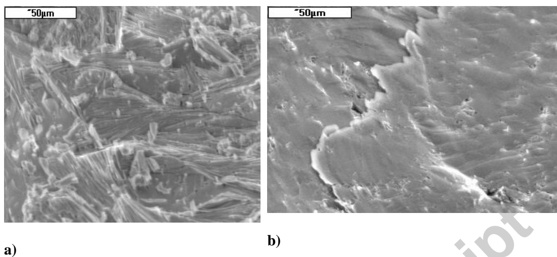
Fig. 1 SEM picture of the fracture of a) \text{AgSbTe}_2 and b) \text{AgSbSe}_2 sample.
