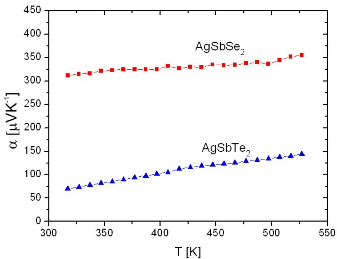
Fig. 3 Temperature dependence of the Seebeck coefficient values of \text{AgSbSe}_2 and \text{AgSbTe}_2 .
