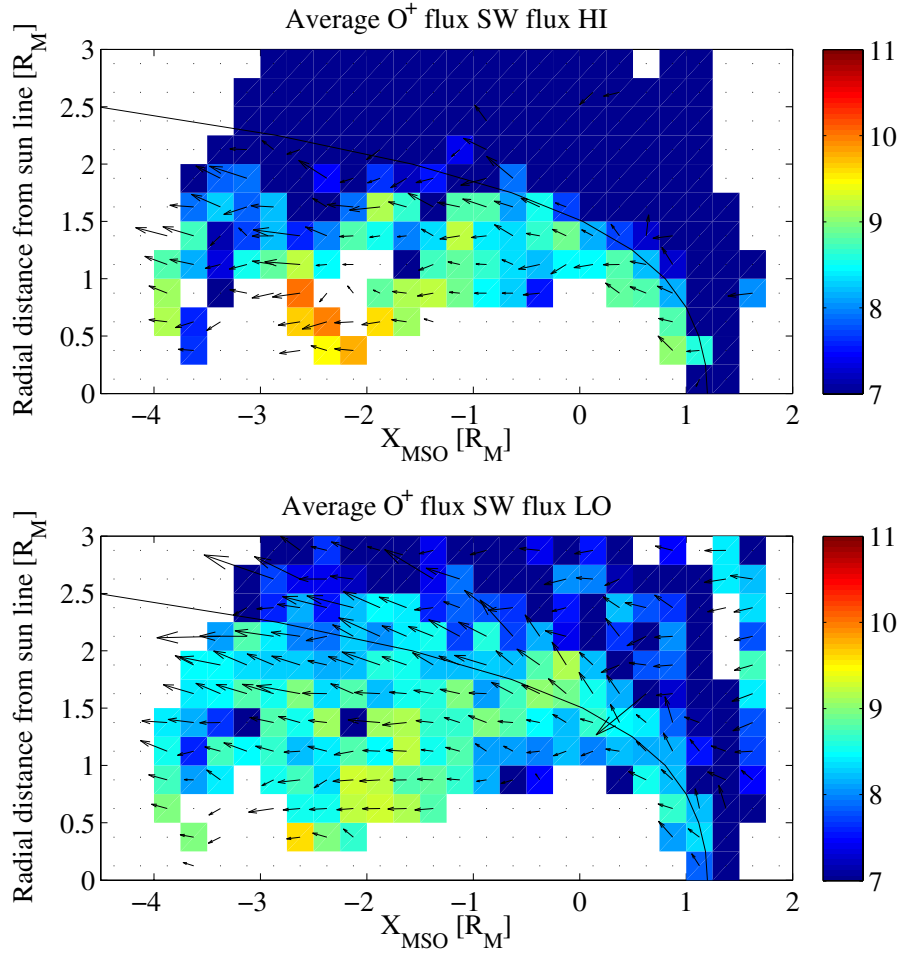
Fig. 6. The colour scale shows the logarithm of average flux of O^+ [ m^{-2} s^{-1} ] for high solar wind flux (upper panel) and low solar wind flux (lower panel). The median value of 4 \cdot 10^{10} m^{-2} s^{-1} solar wind flux density was used to divide the two data sets. The axis are the same as for Fig. 1. Black arrows indicates the average ion bulk velocity, with a scale of 500 km s^{-1}/R_M .
