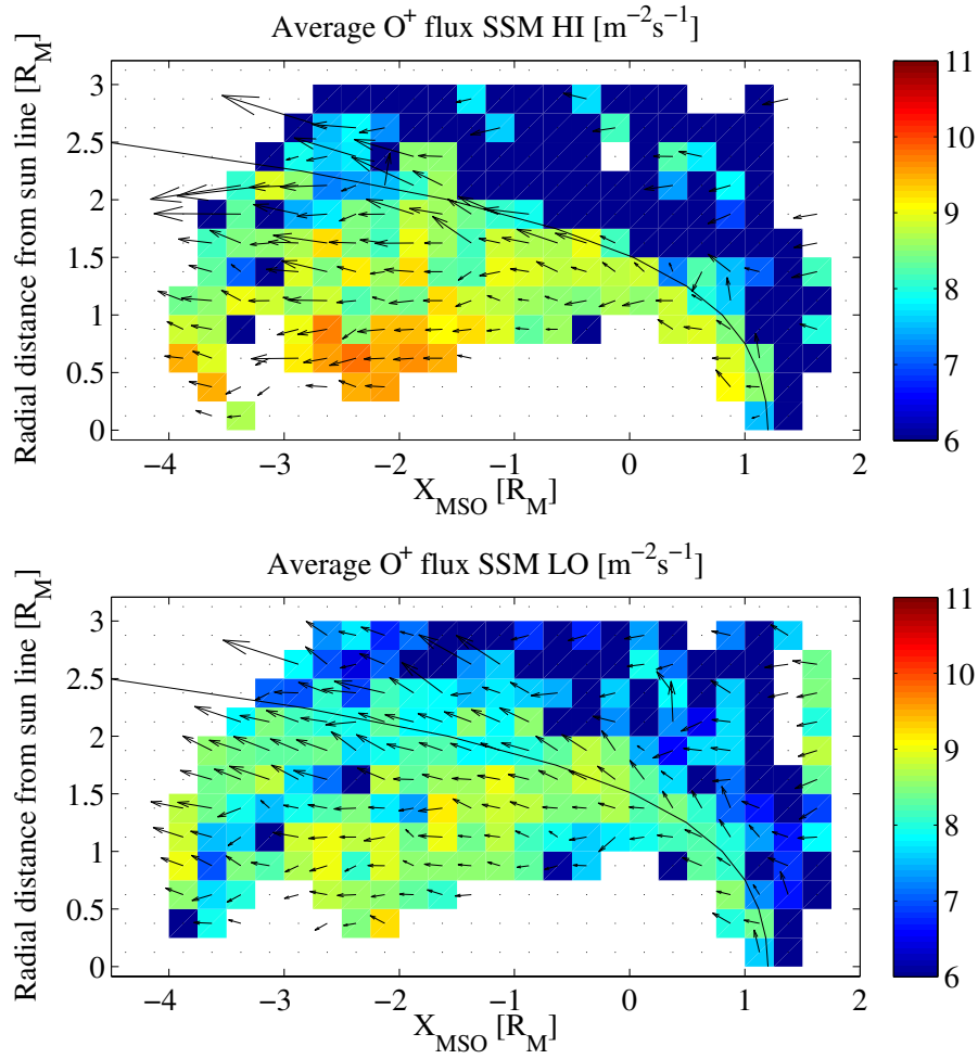
Fig. 5. The colour scale shows the logarithm of average flux of O^+ [ m^{-2} s^{-1} ] for high subsolar magnetic field strength (upper panel) and low subsolar magnetic field strength (lower panel). The median value of 41 nT subsolar magnetic field strength was used to divide the two data sets. The axis are the same as for Fig. 1. Black arrows indicates the average ion bulk velocity, with a scale of 500 km s^{-1}/R_M .
