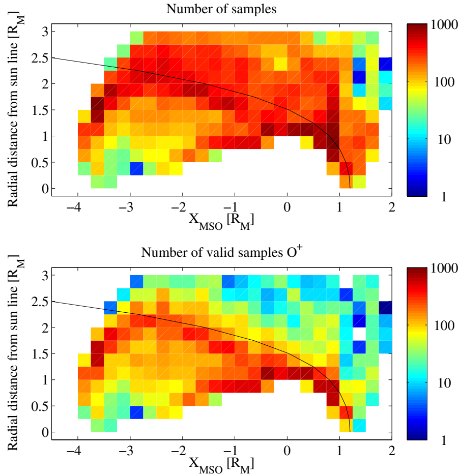
Fig. 2. The colour scale shows the logarithm of the number of samples for all data (upper panel) and with proton and alpha particle flux below a threshold of 10^9 \text{ part. m}^{-2} (lower panel). The axis are the same as for Fig. 1.
