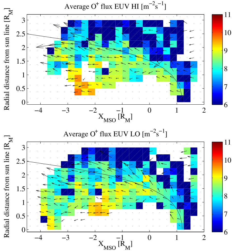
Fig. 4. The colour scale shows the logarithm of average flux of O^+ [ m^{-2} s^{-1} ] for high solar EUV flux (upper panel) and low solar EUV flux (lower panel). The median value of the solar EUV flux of 37 \cdot 10^{-22} W^{-1} m^{-2} Hz^{-1} was used to divide the two data sets. The axis are the same as for Fig. 1. Black arrows indicates the average ion bulk velocity, with a scale of 500 km s^{-1}/R_M .
