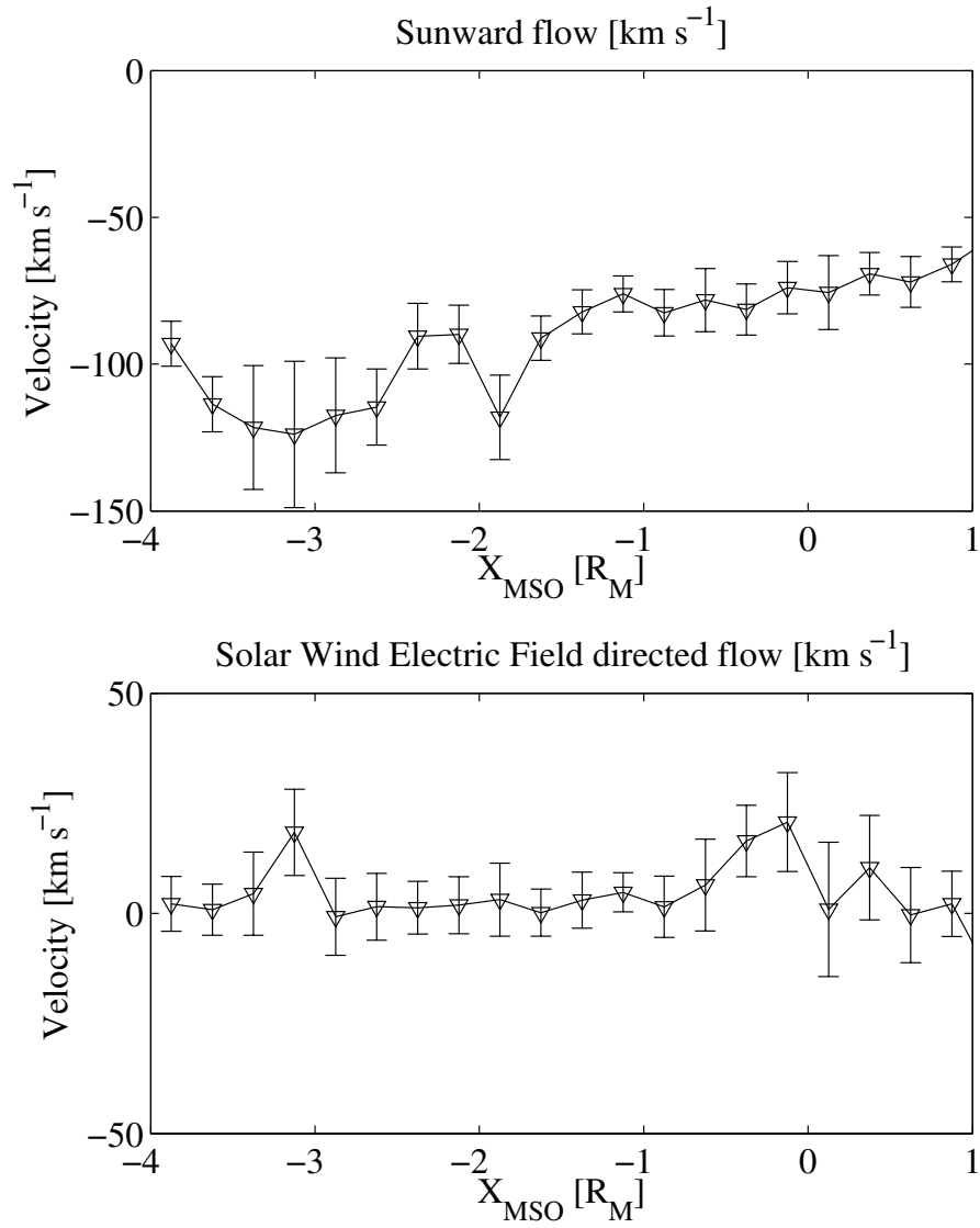
Fig. 9. The x axis shows X_{MSO} distance, positive towards the sun, with Mars center at the origin, in units of Martian radii ( R_M ). The y axis shows the bulk O^+ velocity [ km s^{-1} ] in the sunward direction (panel a) and in the direction of the solar wind electric field (panel b).
