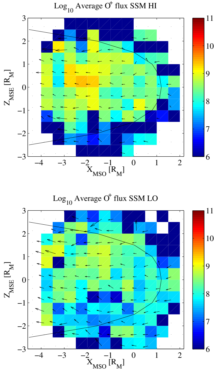
Fig. 8. The colour scale shows the logarithm of average flux of O^+ [ m^{-2} s^{-1} ] for high subsolar magnetic field strength (upper panel) and low subsolar magnetic field strength (lower panel). The median value of 41 nT subsolar magnetic field strength was used to divide the two data sets. The axis are the same as for Fig. 1. Black arrows indicates the average ion bulk velocity, with a scale of 500 \text{ km s}^{-1}/R_M .
