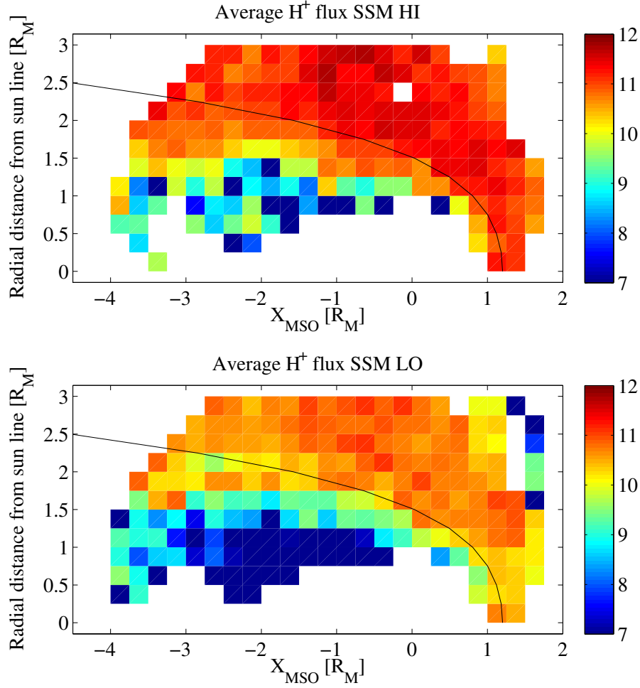
Fig. 1. The colour scale shows the logarithm of average flux of protons [ m^{-2} s^{-1} ] for high subsolar magnetic field strength (upper panel) and low subsolar magnetic field strength (lower panel). The median value of 41 nT subsolar magnetic field strength was used to divide the two data sets. The x axis shows X_{MSO} distance, positive towards the sun, with Mars center at the origin, in units of Martian radii ( R_M ). The y axis shows the radial distance from the X_{MSO} line, i.e. \sqrt{Y_{MSO}^2 + Z_{MSO}^2} in R_M . The thin black line denotes the nominal position of the induced magnetosphere boundary.
