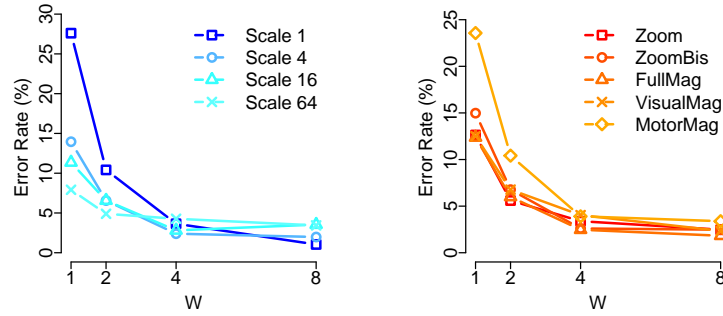
Fig. 10. Error rate as a function of W , for each SCALE (left) and each METHOD (right).
