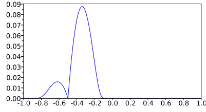
(b) One point EI, EI(x) .
