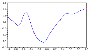
(a) Sample trajectory on 1000 point grid with Matern 5/2 kernel and \theta = 0.3 .
