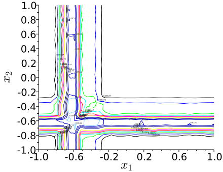
(e) Contour lines of 2 points async. EI (busy point x_{busy} = -0.34 ), EI^{(1,2)}(\mathbf{x})
