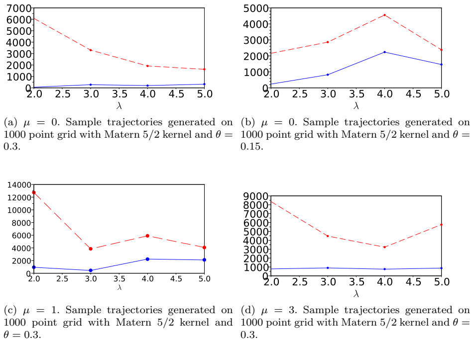
Fig. 6: 80th percentile of the number of MC simulations necessary to discriminate between EI^{(\mu,\lambda)} at two random points versus \lambda . The number of MC simulations without bounds (dashed line), number of MC simulations with bounds (solid line).
