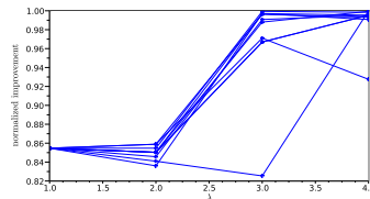
(b) Actual improvement of EI^{(\lambda)} for 10 independent maximizations, \lambda = 1 \dots 4 .
