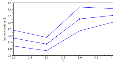
(d) Mean improvement rank, 1\sigma confidence intervals of EI^{(\lambda)} , \lambda = 1 \dots 4 .
