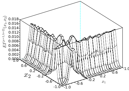
(f) 3D plot of 2 points async. EI (busy point x_{busy} = -0.34 ), EI^{(1,2)}(\mathbf{x})
