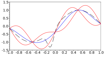
(a) Test function eq. (5) (dashed), kriging model based on 5 observations - predicted mean (blue), 2\sigma predicted confidence intervals (red).
