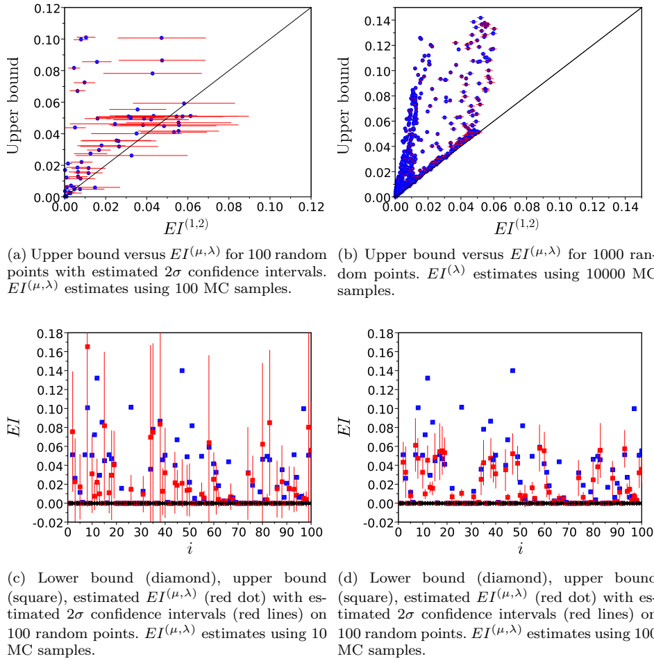
Fig. 5: Upper and lower bounds, EI^{(\mu,\lambda)} ( \mu = 1, \lambda = 2 ) for 100 and 1000 random points with 2\sigma confidence intervals. The test case is based on eq. (5) like in fig. 1. EI^{(\mu,\lambda)} is calculated using 100 and 10000 MC simulations. Notice in this example that for many points the upper bounds are overestimated.
