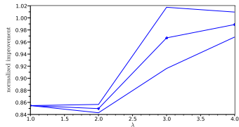
(c) Actual mean improvement, 1\sigma confidence intervals of EI^{(\lambda)} , \lambda = 1 \dots 4 .
