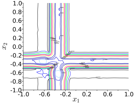
(c) Contour lines of 2 points EI, EI^{(0,2)}(\mathbf{x})
