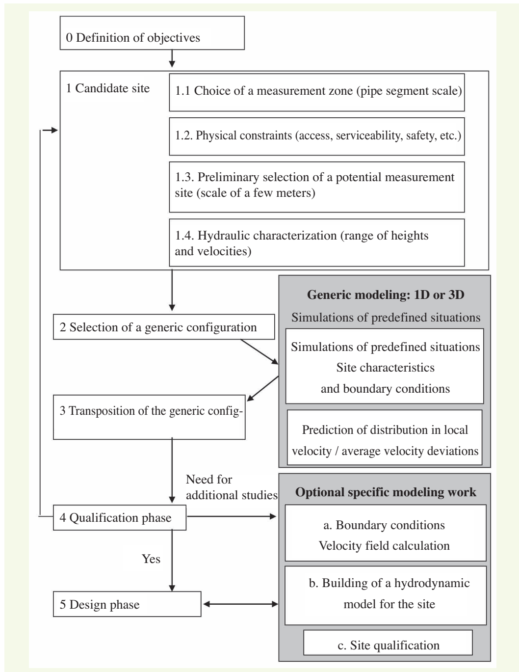
Figure 1 A detailed view of the methodology proposed to qualify a flow meter measurement site and proceed with instrumentation design
