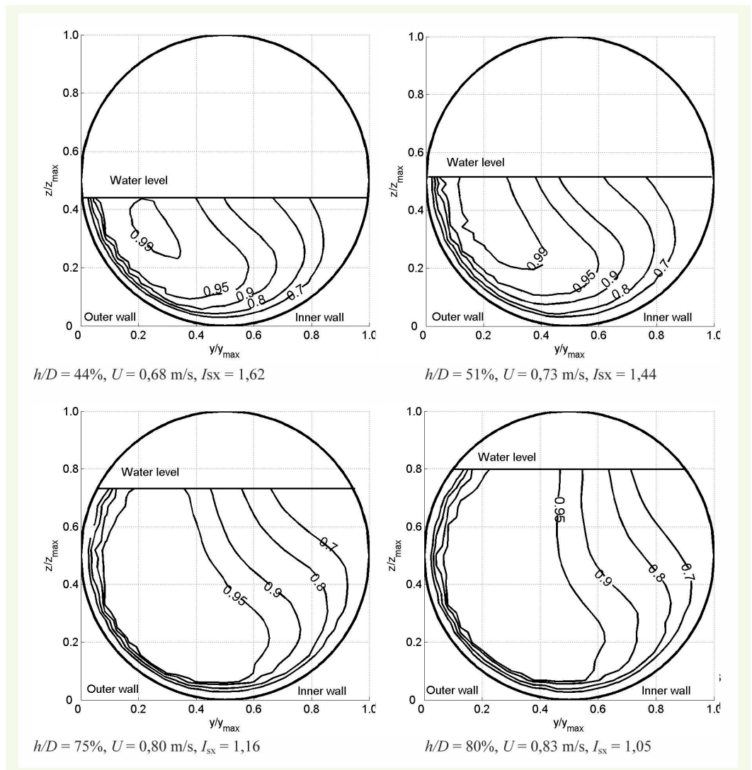
Figure 3 Velocity field U/U_{max} at 10*B downstream of an elbow on a 1.5-m diameter collector for various water levels.
