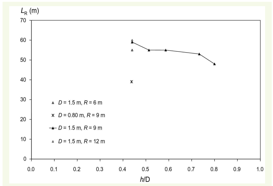
figure 7 Influence of filling rate on the re-establishment length
