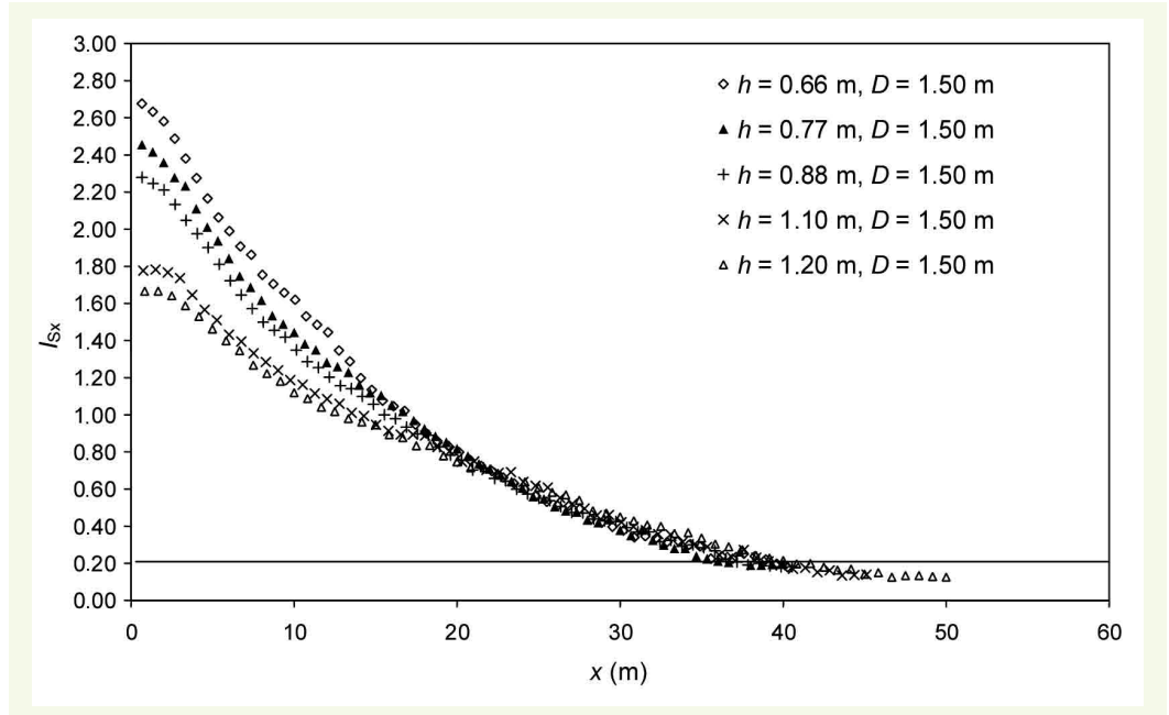
Figure 4 Influence of water height on the singularity index for a collector with a 1.5-m diameter, 9-m radius of curvature and 0.04% slope.
