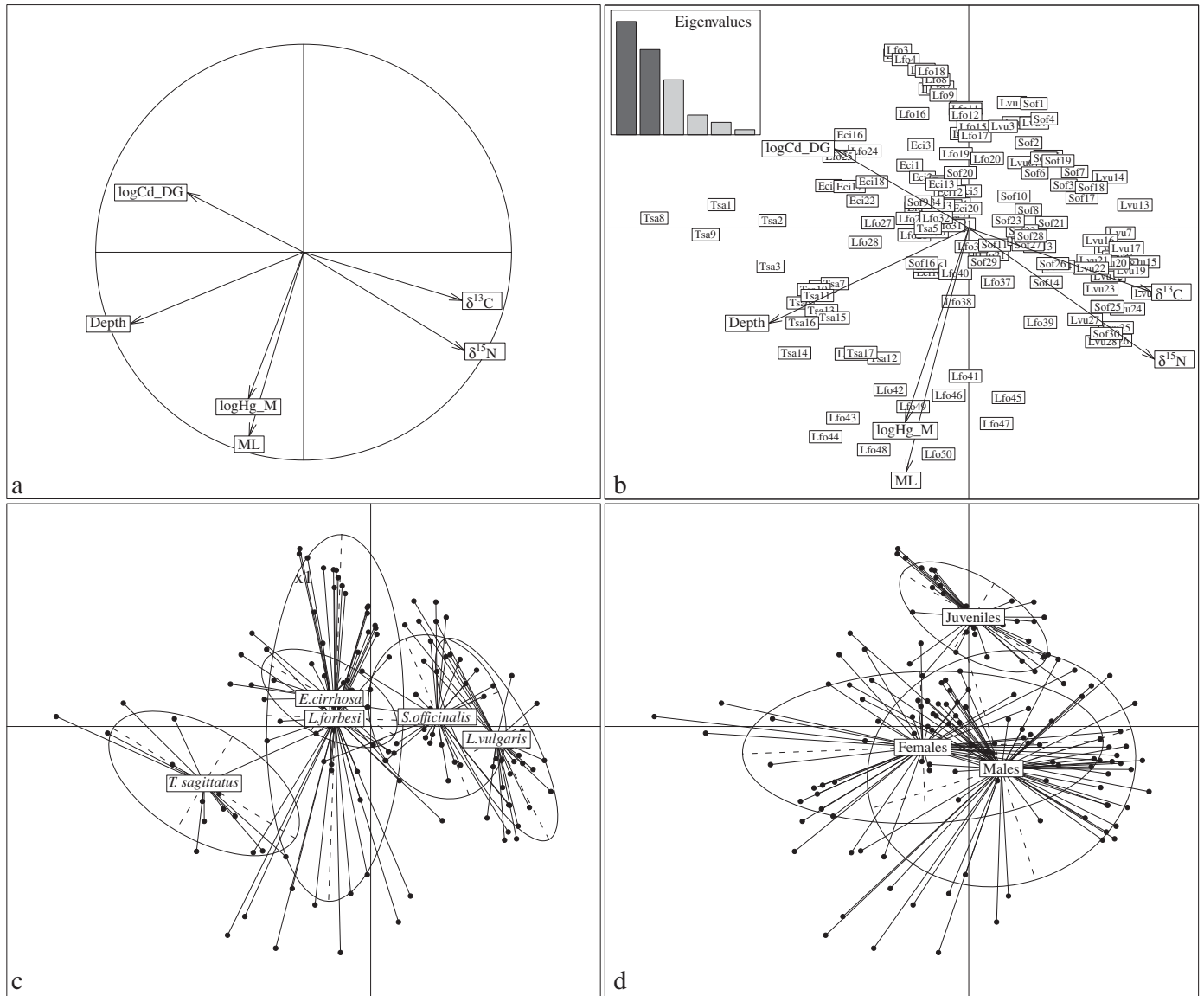
Fig. 2. Eledone cirrhosa , Loligo vulgaris , L. forbesi , Sepia officinalis and Todarodes sagittatus . Projection of variables (Cd DG : Cd in digestive gland; Hg M : Hg in muscle; ML: mantle length) and individuals on the first 2 components resulting from the principal component analysis (PCA). (a) Correlation biplot showing the distribution of the variables. The length of the line for a variable shows how well it is represented by the 2-dimensional approximation, and reflects its contribution to the first 2 principal components. Horizontal axis: principal component 1 (eigenvalue = 2.3, that is 39% of the variability explained by axis 1); vertical axis: principal component 2 (eigenvalue = 1.8, that is 29% of the variability explained by axis 2). Variables pointing in the same direction display a high positive correlation. Variables pointing in the opposite direction have a high negative correlation. Variables with an angle of 90° have a small correlation close to 0. (b) Projection of individuals on the correlation biplot, and histogram of eigenvalues of the different components resulting from the PCA. The black shaded bars refer to the first 2 components with higher eigenvalues, represented on the correlation biplot. The grey shaded bars refer to the other components. Eigenvalues = 2.3, 1.8, 1.1, 0.4, 0.3, 0.1 for the components resulting from the PCA, from 1 to 6 respectively. (c) Grouping of individuals by species. (d) Grouping of individuals by sex (juveniles: small individuals with no visible distinct gonads)
