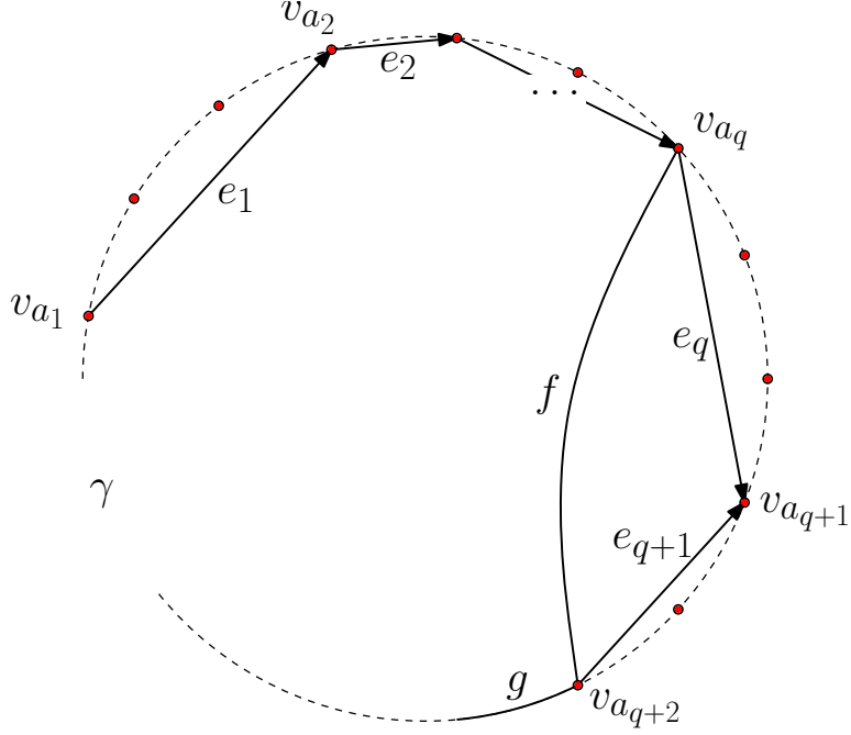
Figure 3: Illustration for the proof of Lemma 9.
