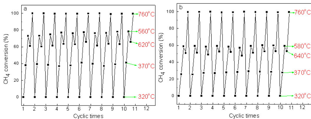
Fig.3 Catalytic stabilities of Pd 0.4 Au 0.2 /SiC (a) and Pd 0.2 Au 0.4 /SiC (b) for methane combustion.
