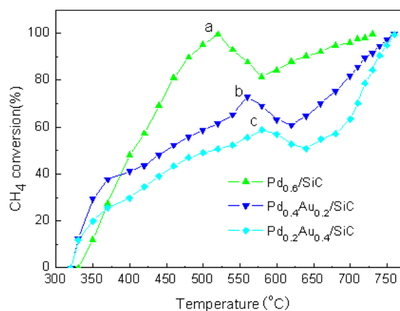
Fig.2 Catalytic activities of Pd 0.6 /SiC, Pd 0.4 Au 0.2 /SiC and Pd 0.2 Au 0.4 /SiC for methane combustion.
