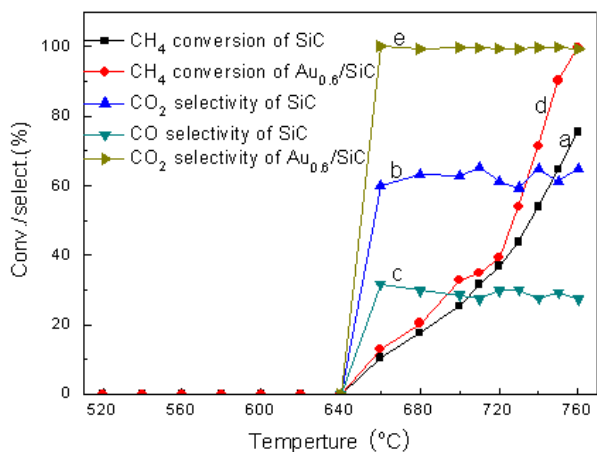
Fig.1 CH 4 conversion and CO 2 selectivity of SiC and Au 0.6 /SiC for methane combustion.
