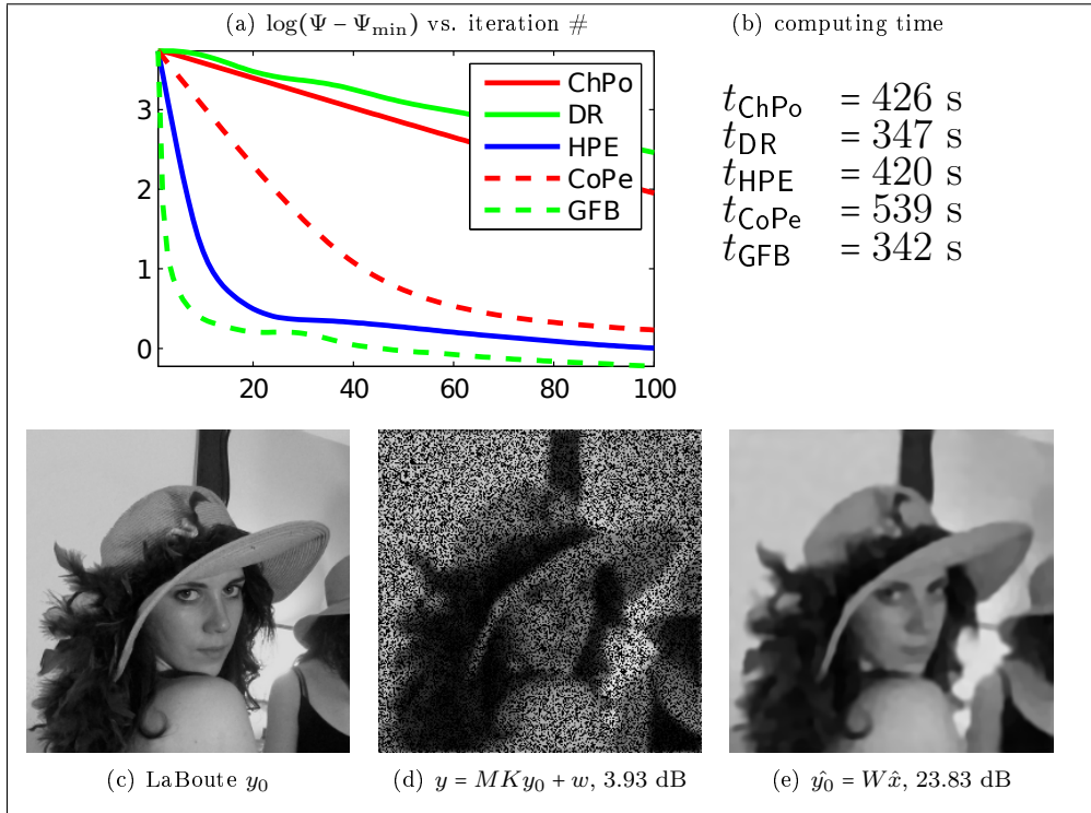
Fig. 7.4: Composite: \sigma = 2 ; \rho = 0.4 ; \mu = 5.0 \cdot 10^{-4} ; S = 4 ; \nu = 5.0 \cdot 10^{-3} .
