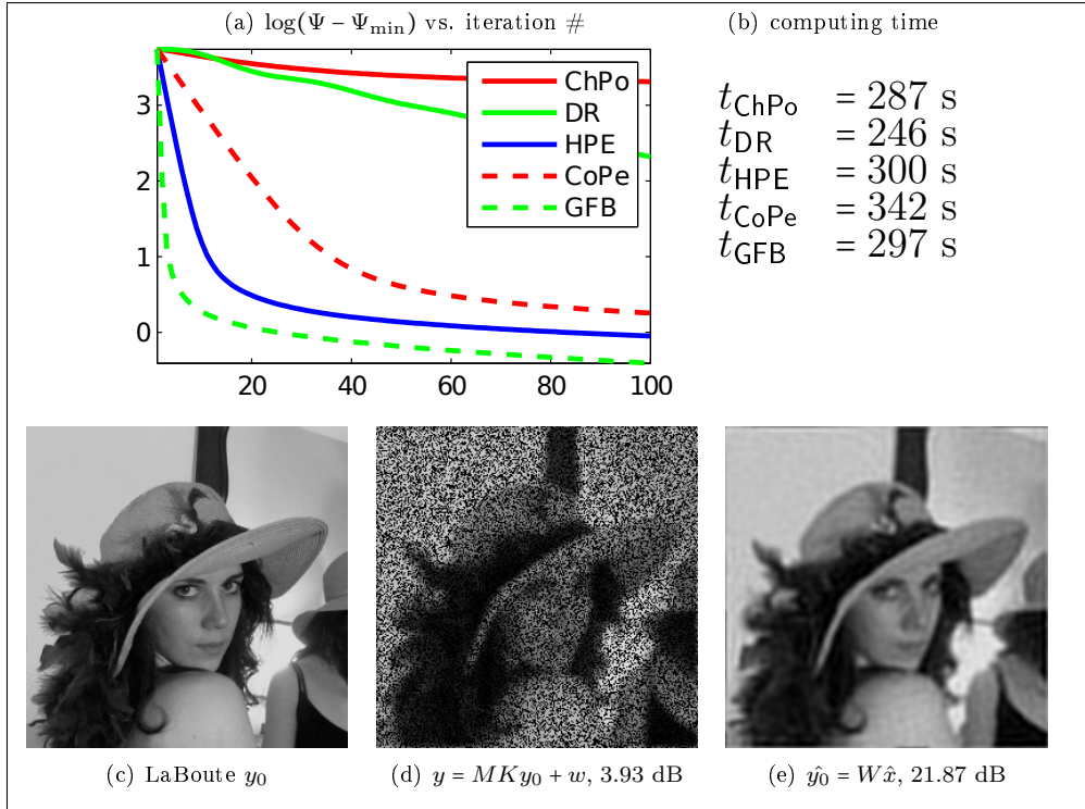
Fig. 7.3: Composite: \sigma = 2 ; \rho = 0.4 ; \mu = 1.0 \cdot 10^{-3} ; S = 4 ; \nu = 0 .
