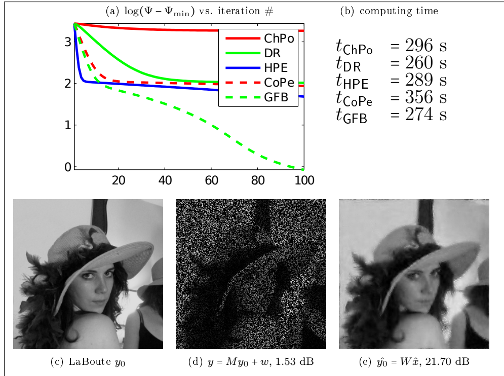
Fig. 7.2: Inpainting: \rho = 0.7 ; \mu = 2.6 \cdot 10^{-3} ; S = 4 ; \nu = 0 .
