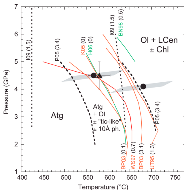
Figure 3. P, T conditions for antigorite dehydration. Solid red lines locate the stability limit of antigorite measured in quench studies by WS97 [Wunder and Schreyer, 1997], BP03 [Bromiley and Pawley, 2003], UT95 [Ulmer and Trommsdorff, 1995], and K05 [Komabayashi et al., 2005]. Solid green lines locate the stability limit of antigorite calculated by H06 [Hilairat et al., 2006] and BN98 [Bose and Navrotsky, 1998]. The fields of the “talc-like” phase, observed by P05 [Perrillat et al., 2005] and I09 [Inoue et al., 2009], are reported by dashed lines. The \text{Al}_2\text{O}_3 content of antigorite is given in parentheses. Solid circles show the onset of steps 1 and 2 of the reaction observed during the present in situ experiment. The parallelograms of uncertainties on (P, T) conditions are also reported. The triangle locates (P, T) conditions of the off-line experiment. Atg, for antigorite; talc-like, the talc-like phase; 10 Å ph., 10 Å phase; Ol, olivine; LCen, low clinoenstatite; and Chl, chlorite.
