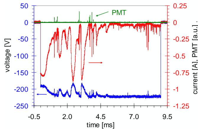
Figure 2.4. The measured current and voltage time dependence of the system during a 9 ms, -225 V pulse with liquid at room temperature ( \sim 20^{\circ}\text{C} ). Also shown is the response of a fast photomultiplier tube (PMT) viewing the electrode tip region [from Schaper et al. 2010b].
