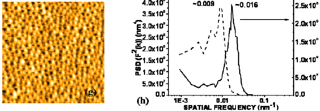
Figure 6. Plasma directed organization on PMMA film in O_2 plasma and the role of reactor walls. AFM images ( 2 \times 2 \mu m ) are shown. Typical etch rates are 600 nm/min, while nanodot formation is observed only at certain wall conditions.
