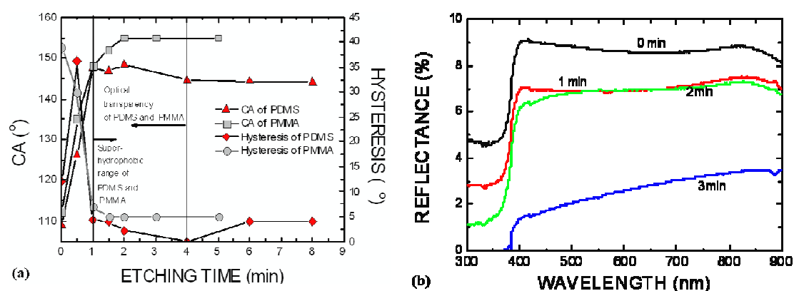
Figure 9. (a) CA and CA hysteresis versus etching time for PDMS and PMMA. The evolution of super-hydrophobicity and the process window for optical transparency are also indicated. (b) Reflection spectra (at 6°) of 2mm PMMA substrates before and after 1, 2, 3 min O 2 plasma processing on ONE side of the polymer plate only(9).
