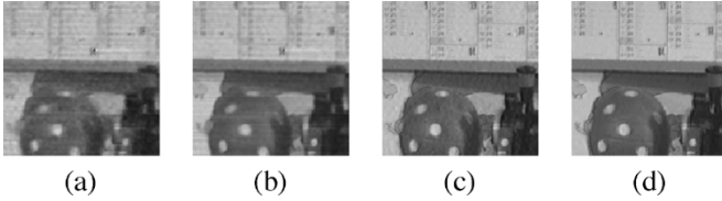
Fig. 9. Output of filtered Caltrain third frame 256 \times 256 corrupted by mixed impulsive ( p = 5\% ) and Gaussian additive noise ( \sigma = 20 ): (a) 3-D NLMS L -filter with ( \mu_0 = 0.8 ), (b) 3-D recursive NLMS L -filter with ( \mu_0 = 0.8 ), (c) 3-D NLMK L -filter with ( \mu_0 = 10^{-4} ), and (d) 3-D recursive NLMK L -filter with ( \mu_0 = 10^{-4} ).
