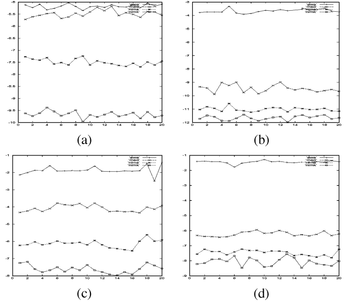
Fig. 5. SNRI improvements versus frame numbers. (a) Trevor sequence with mixed noise ( \sigma = 20, p = 5\% ). (b) Trevor sequence with salt and pepper noise ( p = 10\% ). (c) Caltrain sequence with mixed noise ( \sigma = 20, p = 5\% ). (d) Caltrain sequence with salt and pepper noise ( p = 10\% ).
