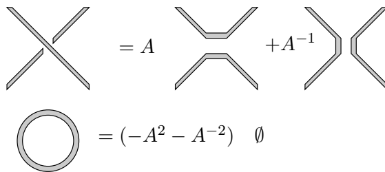
Figure 4: Kauffman relations
