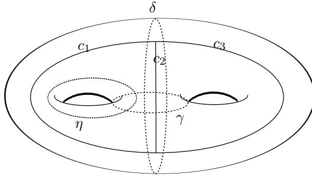
Figure 10: Curves on a genus 2 surface
