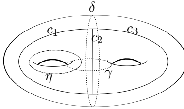
Figure 2: Curves on a genus 2 surface
