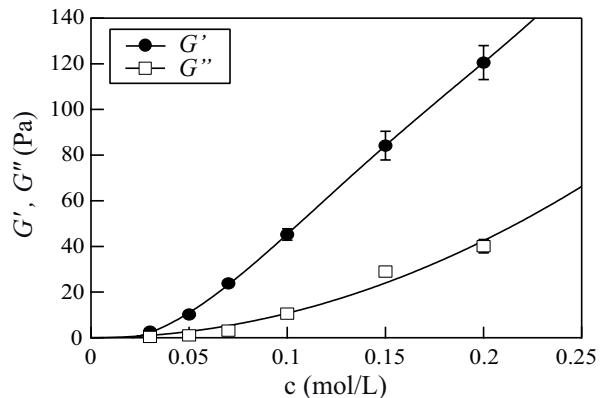
FIG. 11. Average elastic ( G' ) and viscous ( G'' ) moduli corresponding to the plateau value in Fig. 10] as a function of the fluid concentration. Lines are given as eyeleads.
