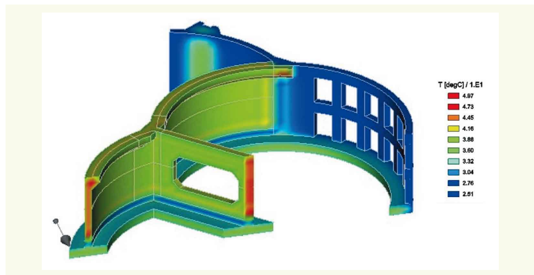
Figure 6 Temperature iso-values
