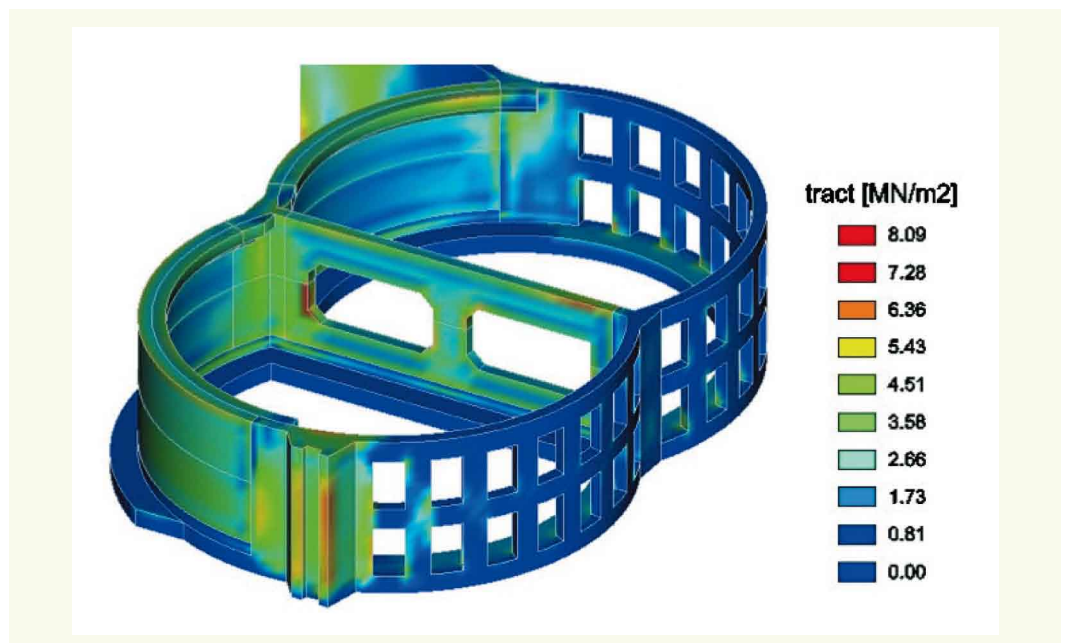
Figure 8 Tensile stress iso-values
