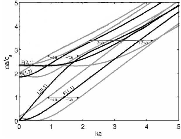
Figure 4: Wavenumber translation for some examples of F(m,n) modes (same legend as Fig. 3). The wavenumber of the L(0,1) mode is left unchanged (axisymmetric mode).
