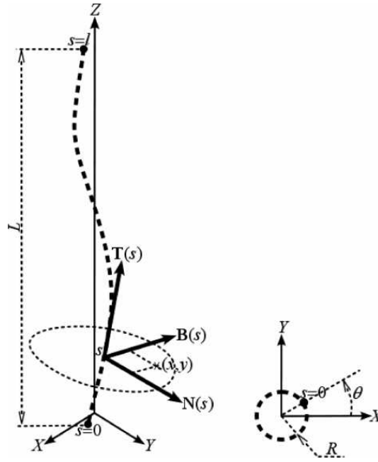
Figure 1: Left: helix centreline curve (one step) with its associated Serret-Frenet basis and (x, y, s) helical coordinate system. Right: plane view. The point s = 0 lies in the (X, Y) plane.
