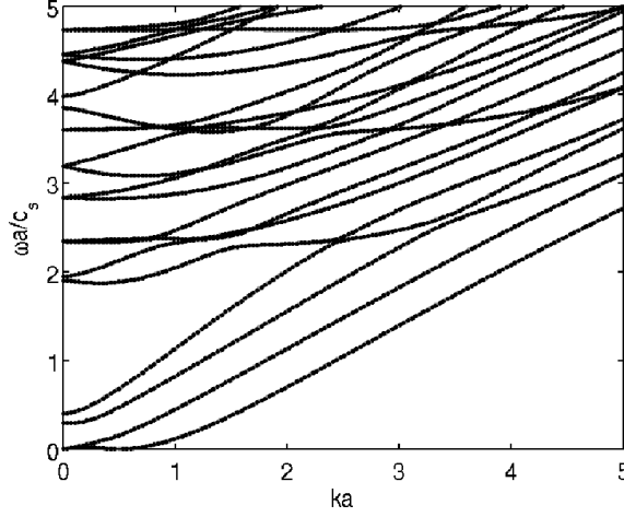
Figure 6: Plot of normalized frequency vs. wavenumber for the helical waveguide R = 2a , \phi = \pi/4 . Black: helical system (reference), gray: twisting system.
