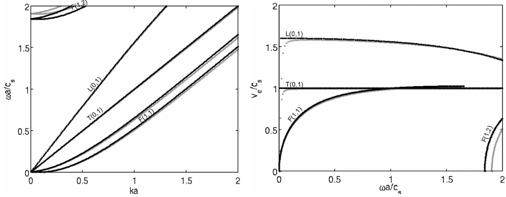
Figure 8: Dispersion curves for single wires. Black: central wire, gray: peripheral wire. Left: plot of normalized frequency vs. wavenumber, right: plot of normalized energy velocity vs. frequency.
