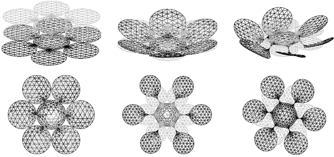
Figure 11: From left to right: real part (top) and imaginary part (bottom) of the displacement modeshape of branch 1 computed at points 1a, 1b and 1c (located in Fig. 10). Gray meshes correspond to the undeformed cross-section. The view of imaginary part is 2D for clarity.
