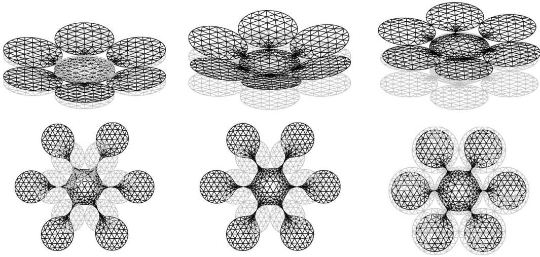
Figure 12: From left to right: real part (top) and imaginary part (bottom) of the displacement modeshape of branch 2 computed at points 2a, 2b and 2c (located in Fig. 10). Gray meshes correspond to the undeformed cross-section. The view of imaginary part is 2D for clarity.
