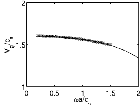
Figure 13: Central wire (cylindrical). Normalized group velocity vs. frequency measured with the magnetostrictive device (x-mark) and computed with the SAFE model (solid line) for the L(0,1) mode.
