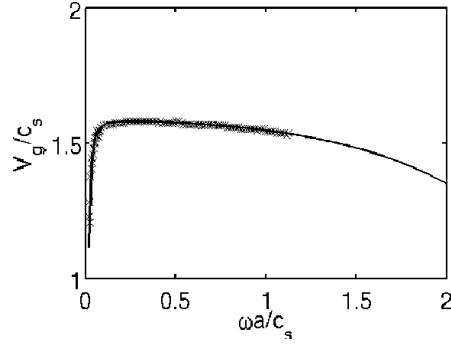
Figure 14: Peripheral wire (helical). Normalized group velocity vs. frequency measured with the magnetostrictive device (x-mark) and computed with the SAFE model (solid line) for the L(0,1) mode.
