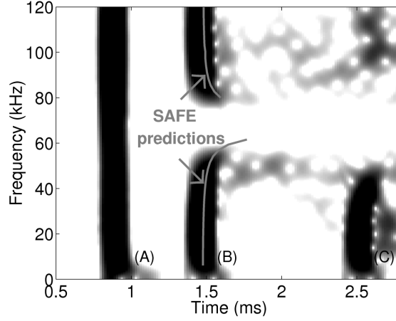
Figure 15: Seven-wire strand. SAFE predictions (gray solid lines) of group-time delays for the compressional-like L(0,1) modes superimposed to the experimental spectrogram. (A), (B) and (C) respectively denote the arrivals related to the electro-magnetic coupling between coils, the direct mechanical wave and the first reflection of the direct wave.
