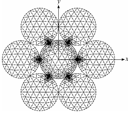
Figure 7: Cross-section FE mesh for the seven-wire strand \phi = 7.9^\circ (6975 dofs).
