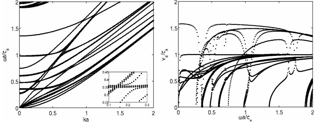
Figure 9: Dispersion curves for the seven-wire strand. Left: plot of normalized frequency vs. wavenumber (inset: zoom on the veering region of compressional-like L(0,1) modes), right: plot of normalized energy velocity vs. frequency.
