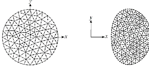
Figure 2: Left: cross-section FE mesh of a cylindrical waveguide (and of a helical waveguide analysed with the helical coordinate system). Right: cross-section FE mesh of a helical waveguide R = 2a , \phi = \pi/4 analysed with the twisting coordinate system.
