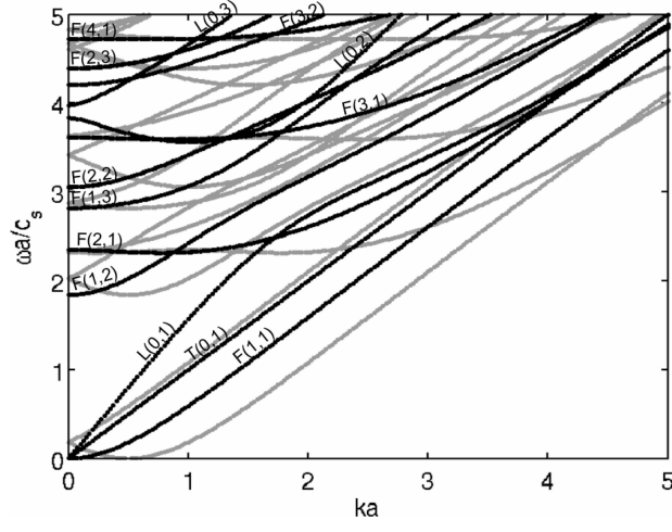
Figure 3: Plot of normalized frequency vs. wavenumber for a cylindrical waveguide. Black: Cartesian system (reference), gray: twisting system.
