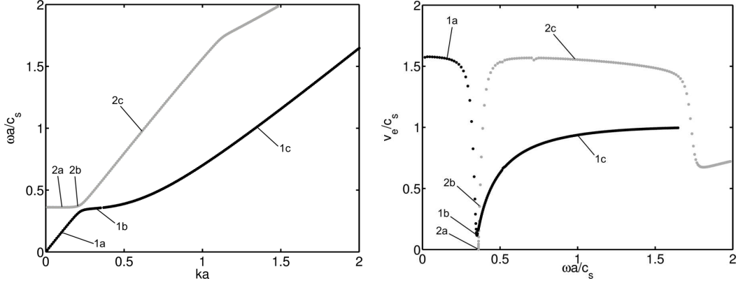
Figure 10: Branch identification of compressional-like L(0,1) modes for the seven-wire strand (black: branch 1, gray: branch 2). Left: plot of normalized frequency vs. wavenumber. Right: plot of normalized energy velocity vs. frequency. The modes shapes corresponding to points 1a, 1b and 1c are given by Fig. 11, those corresponding to 2a, 2b and 2c are given by Fig. 12.
