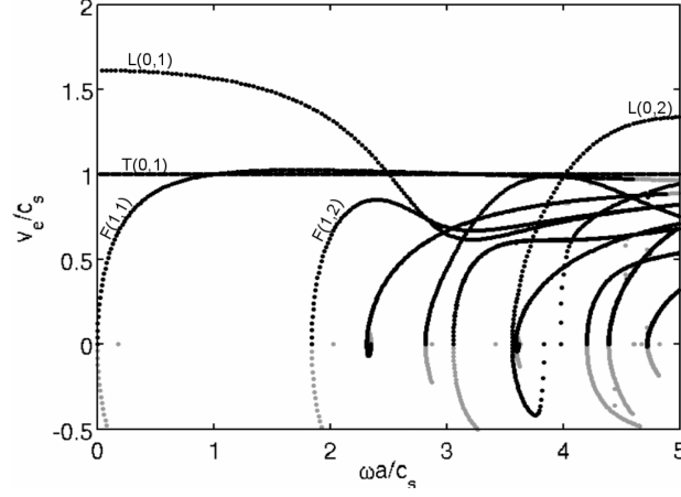
Figure 5: Plot of normalized frequency vs. wavenumber for a cylindrical waveguide. Black: Cartesian system (reference), gray: twisting system.
