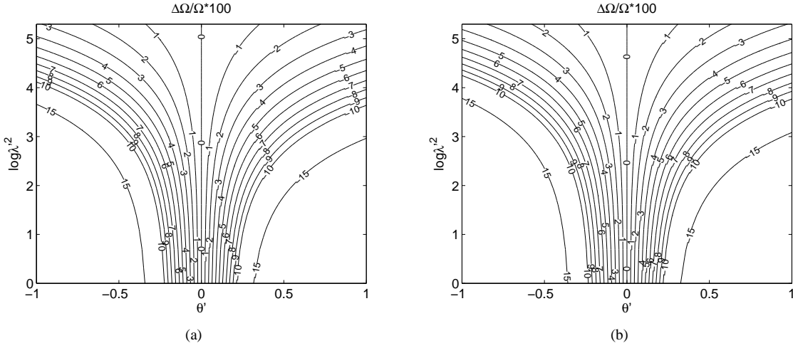
Figure 10: Relative change in natural frequency (x100) of the 1st antisymmetric mode for \xi = 300 (a) and \xi = 50 (b).
