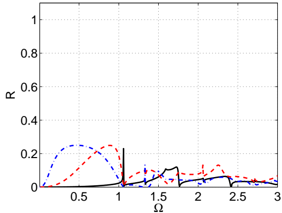
Figure 10: Power reflection coefficient of the flexural mode F(1,1) when the T(0,1) mode encounters a crack with depths d = 0.5r (—), d = 1.0r (---) and d = 1.5r (-·-).
