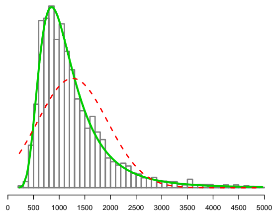
Figure 8. Typical distribution of movement time for a percentile interval ( 3.6 \leq ID_{min} \leq 3.85 , 3179 values) for configuration # 17. The dashed (red) line is the normal fit (mean 1271, deviation 696) and the plain (green) one is the gev fit (location 931, scale 391 and shape 0.24).
