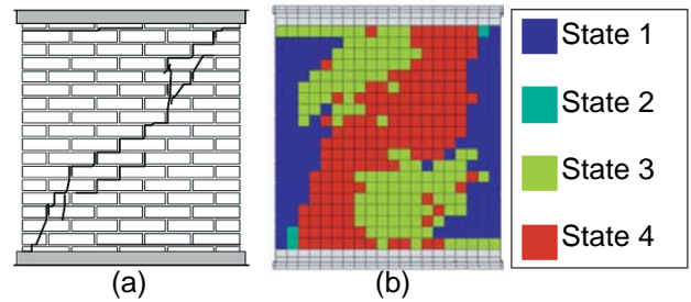
Figure 11: Crack patterns comparison: (a) Experimental result; (b) Numerical result.
