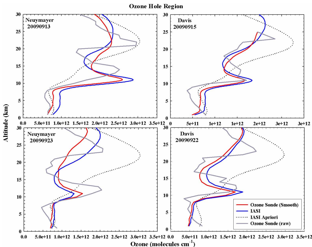
Fig. 12. Comparisons between IASI and ozone sonde profiles measured within the ozone hole at the Neumayer (left) and Davis (right) stations for different days of September 2009. The IASI a priori is represented by the black dotted line. The IASI profile is an averaged profile of between 5 and 10 profiles (depending on the location), co-located in time and space to the ozone sonde measurements (raw data interpolated at the IASI altitude). The ozone sonde profile (in grey) has been convolved with the IASI averaging kernels (in red). Note that the a priori profile here has been converted from mixing ratios (independent of temperature and pressure) to density (dependent on temperature and pressure). Thus if temperature and pressure change from one location or day to another, different a priori profiles in density will be found.
