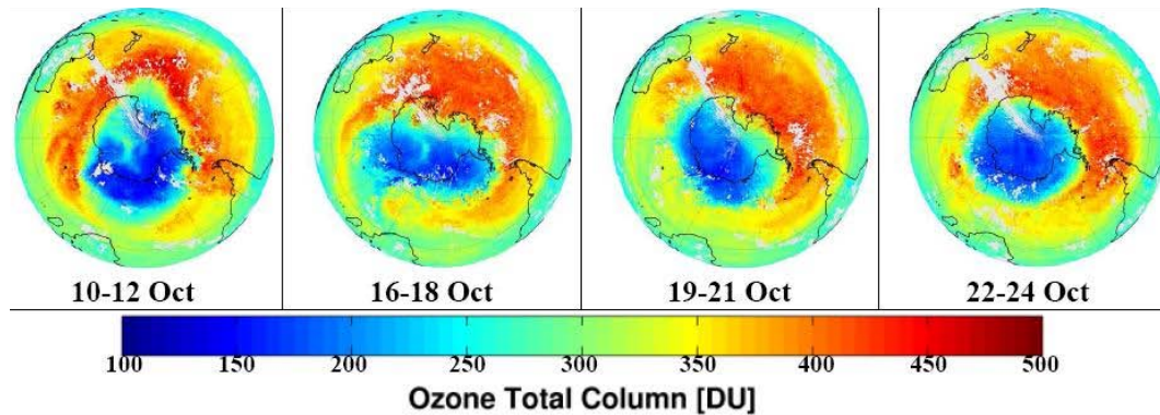
Fig. 7. Total ozone column distributions above Antarctica averaged over 3 day periods in October 2009. The change from a circular to elliptical rotation and back again is clearly visible. Data are averaged over a 1^\circ \times 1^\circ grid.
