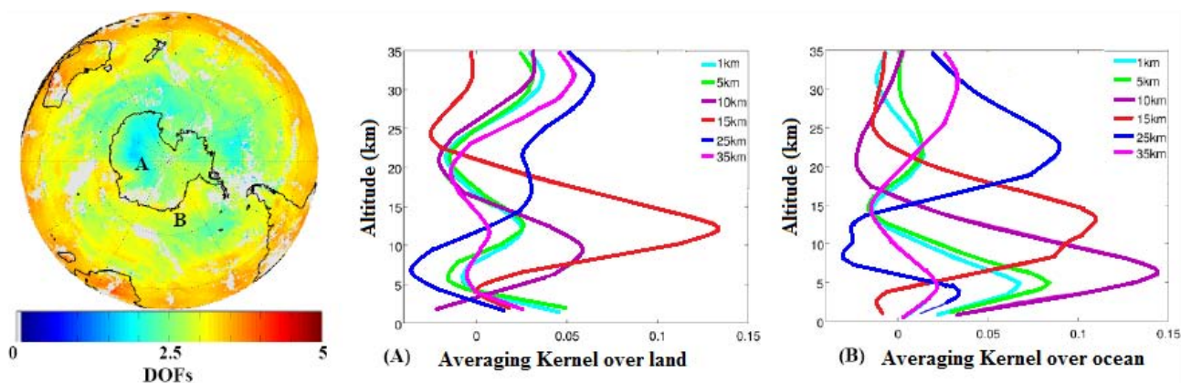
Fig. 4. IASI DOFs distribution above Antarctica (grey is for no data), along with averaging kernel functions for partial columns of different altitudes characterizing the retrievals from spectra shown in Fig. 3, over land (A) and over ocean (B), respectively.
