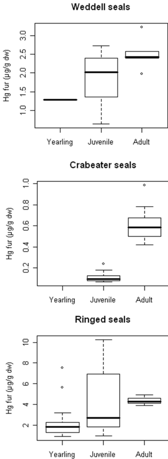
Fig. 2 Comparisons of Hg concentrations in fur (in \mu\text{g/g dw} ) among age classes for the Weddell seals, crabeater seals and ringed seals. The upper and lower hinges represent the quartiles, the vertical lines, the maximum and minimum data values and the bold line represents the median value while the points are outliers
