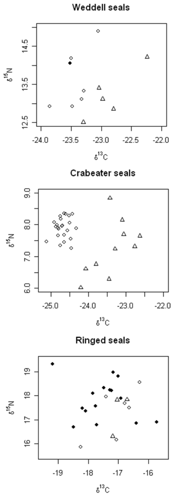
Fig. 3 Relations between \delta^{15}\text{N} (‰) vs \delta^{13}\text{C} (‰) values for the three age classes (filled circle = yearling, open circle = juvenile, open triangle = adult) for the Weddell seals, crabeater seals and ringed seals
