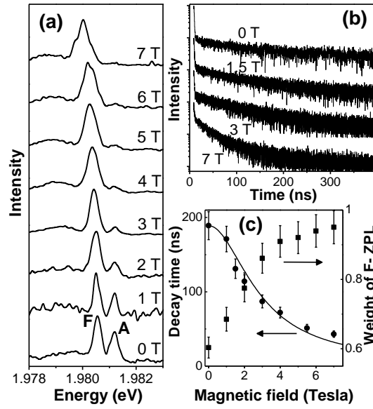
Fig. 1: (a) PL spectra of a single NC in a magnetic field nearly perpendicular to the c -axis. The lines labelled A and F are the recombination ZPLs of the bright and the dark excitons, respectively. (b) PL decay of this NC for various intensities of the magnetic field. (c) Circles: Field-induced shortening of the PL long decay time. The solid curve is a fit which leads to the relative angle \theta = (75 \pm 5)^\circ between the NC c -axis and the field, taking \tau_0 = 2 ns and \tau_F(0) = 190 ns in expression (1). Squares: Relative weight of the F line in the ZPL structure, as a function of the magnetic field.
