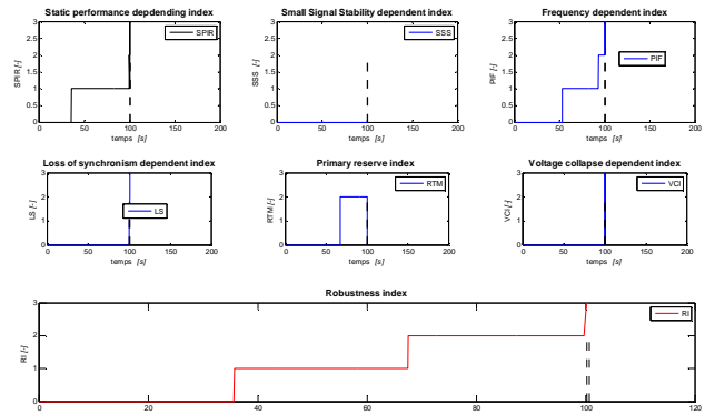
Fig.8. Robustness index in abnormal state
