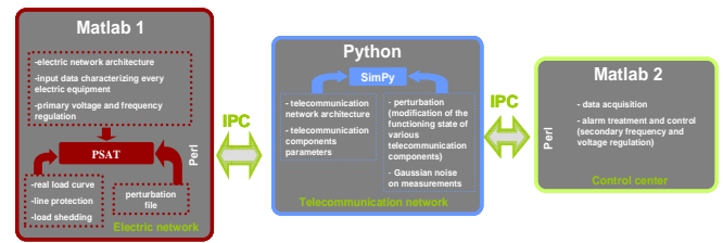
Fig. 3. The combined simulator
