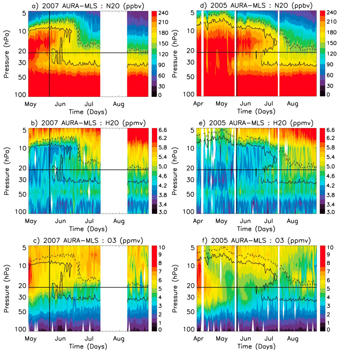
Figure 3. Time evolution of vertical profiles of N 2 O, H 2 O and O 3 volume mixing ratios inside the FrIAC cores in (a, b, c) 2007 and (d, e, f) 2005 obtained from the AURA-MLS instrument. The daily vertical profiles were selected using the criterion of maximum mixing ratio of N 2 O northward of 60°N for each MLS pressure level in the range [100–5] hPa. The black and dashed isocontours displayed on each figure correspond to 180 ppbv and 140 ppbv N 2 O respectively. The vertical black solid line corresponds to the transition between the “anticyclonic phase” and the “shearing phase,” in 2007 and 2005. The horizontal black solid line depicts the lowest MLS level where the FrIACs have been detected (21.5 hPa). White areas indicate a lack of data.
