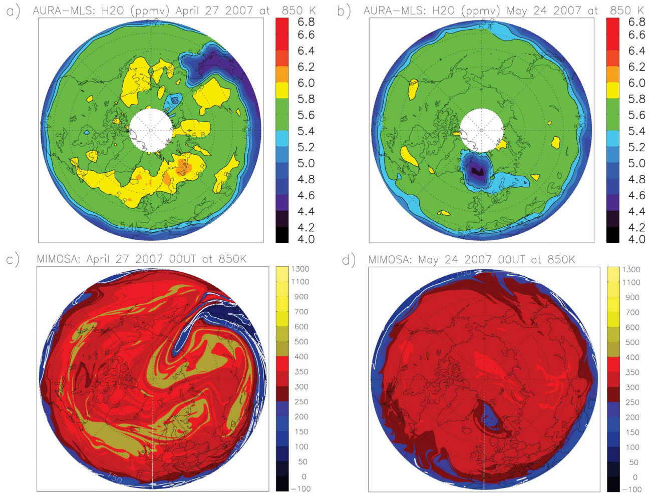
Figure 1. (a, b) Isocontours of water vapor mixing ratio (ppmv) from the MLS instrument interpolated on the 850K isentropic surface and (c, d) potential vorticity maps simulated by MIMOSA model. Figures 1a and 1c show 27 April 2007 during the intrusion leading to the FrIAC. Figures 1b and 1d show 24 May 2007 when the FrIAC is trapped at high latitudes. In Figure 1 and in remaining figures, potential vorticity is plotted in pvu ( 10^{-6} \text{ km}^2 \text{ kg}^{-1} \text{ s}^{-1} ).
