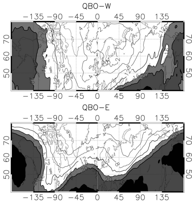
Figure 11. Frequency of occurrence (in percent) of air mass with PV lower than the zonal-mean PV at 30^{\circ}\text{N} and 850\text{ K} during January/February for the QBO westerly phase (years 2002, 2004, 2006, 2008) on the top and the QBO easterly phase (years 2000, 2003, 2005, 2007, 2009) on bottom. Dark contours are for frequencies higher than 16%.
